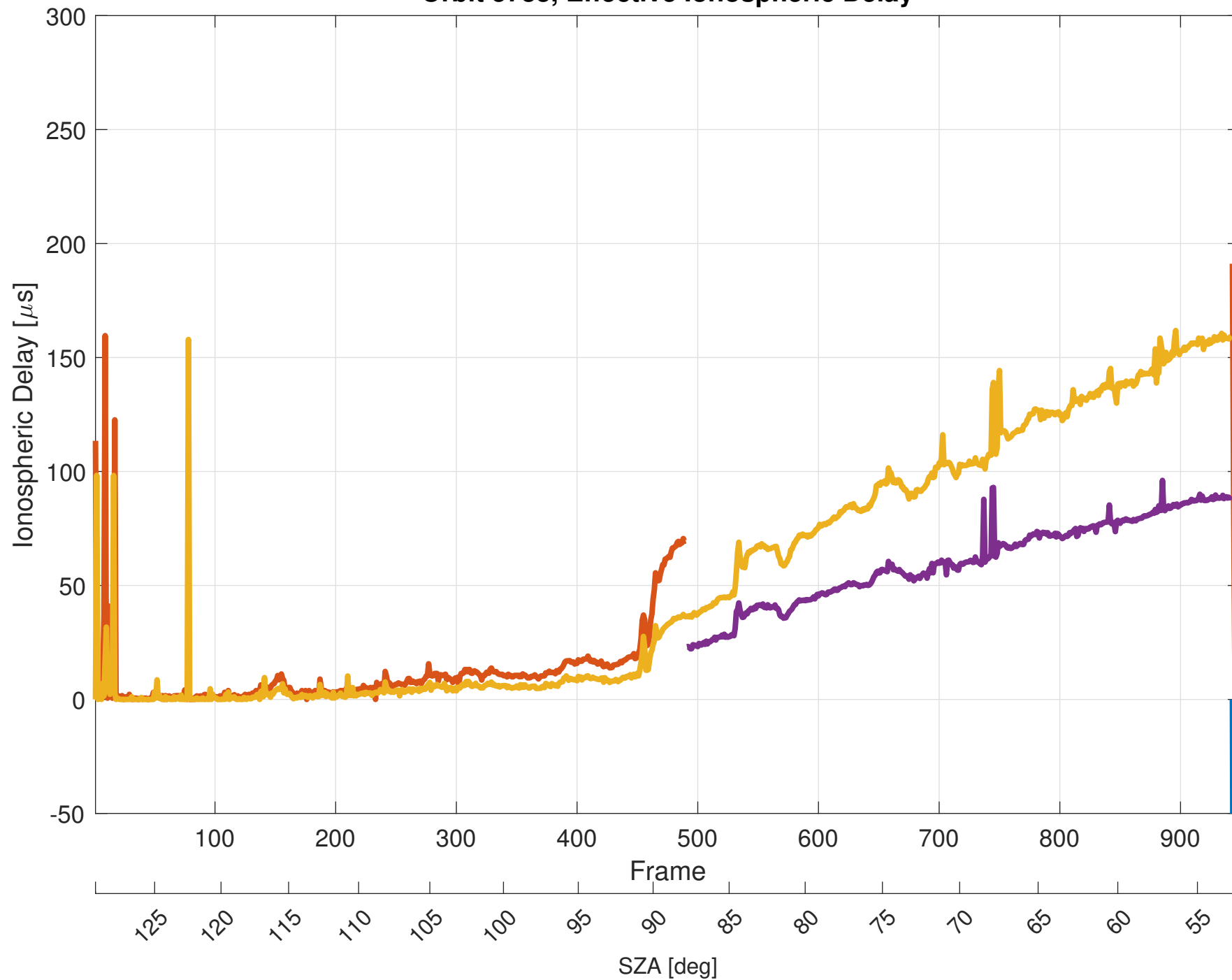
Orbit 5733, Effective Ionospheric Delay
