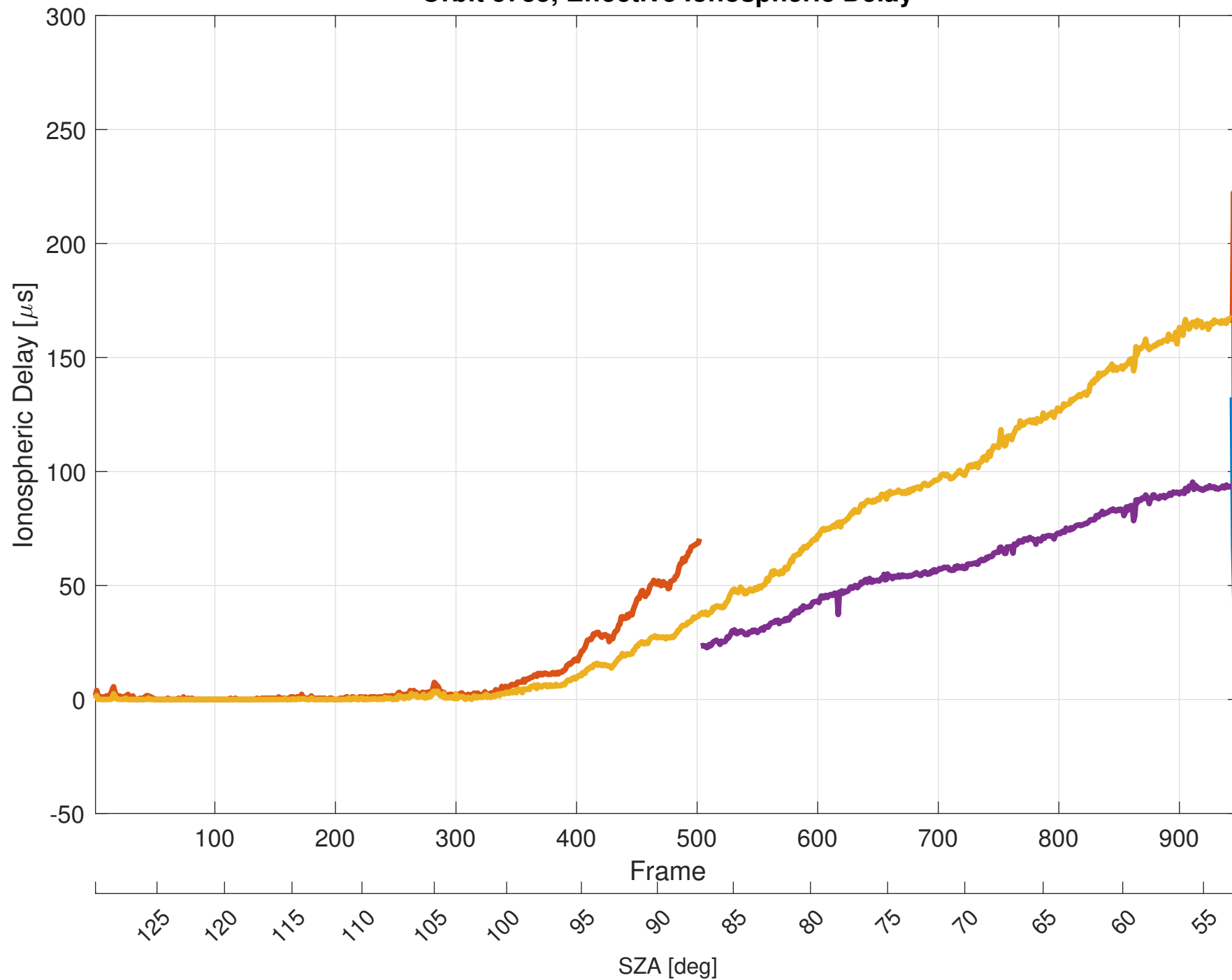
Orbit 5735, Effective Ionospheric Delay
