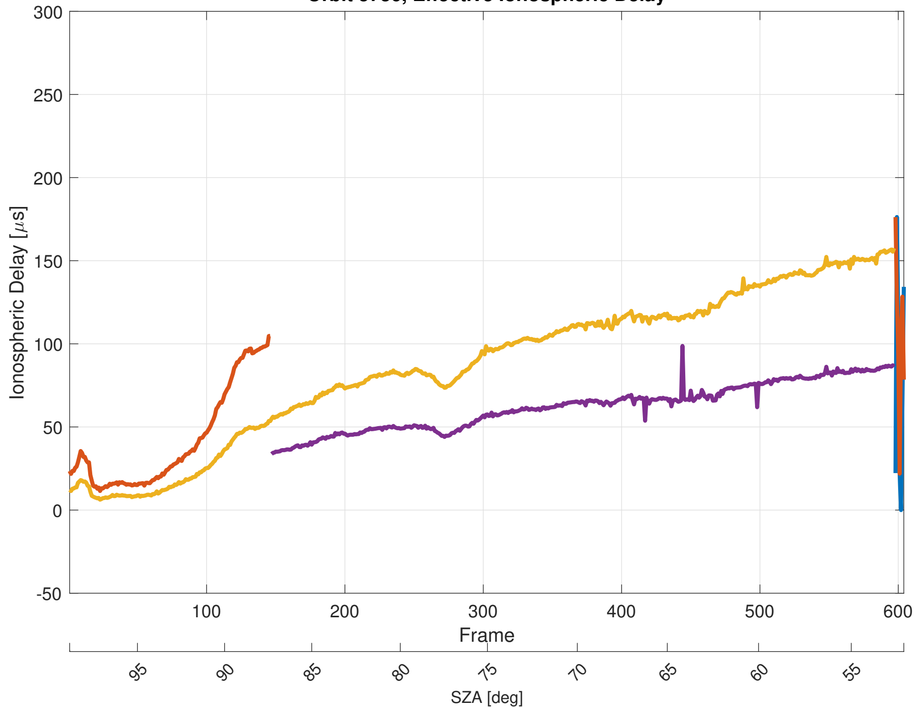
Orbit 5736, Effective Ionospheric Delay
