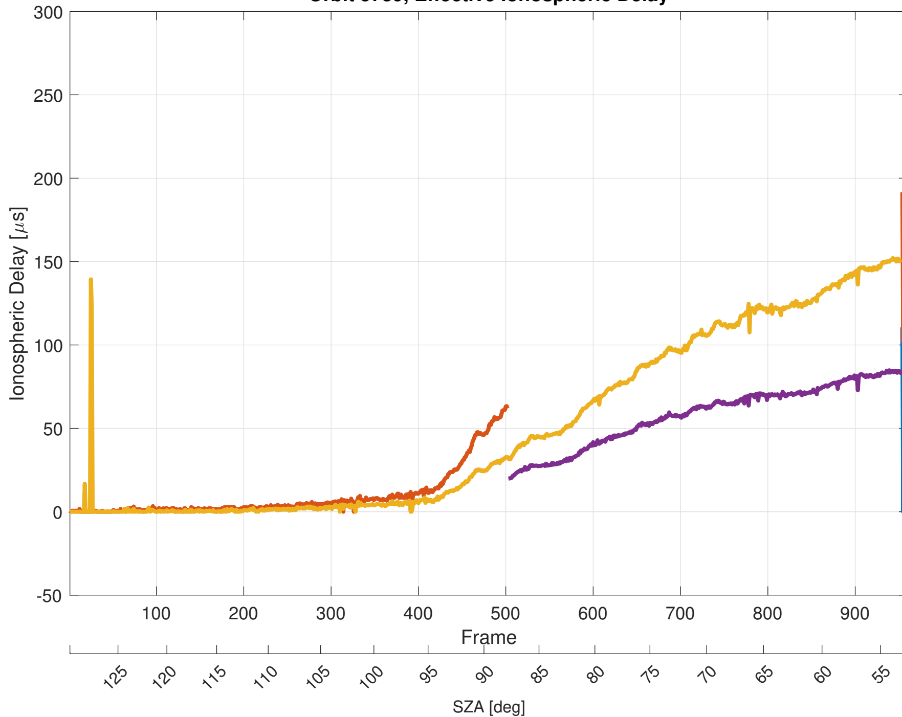
Orbit 5739, Effective Ionospheric Delay
