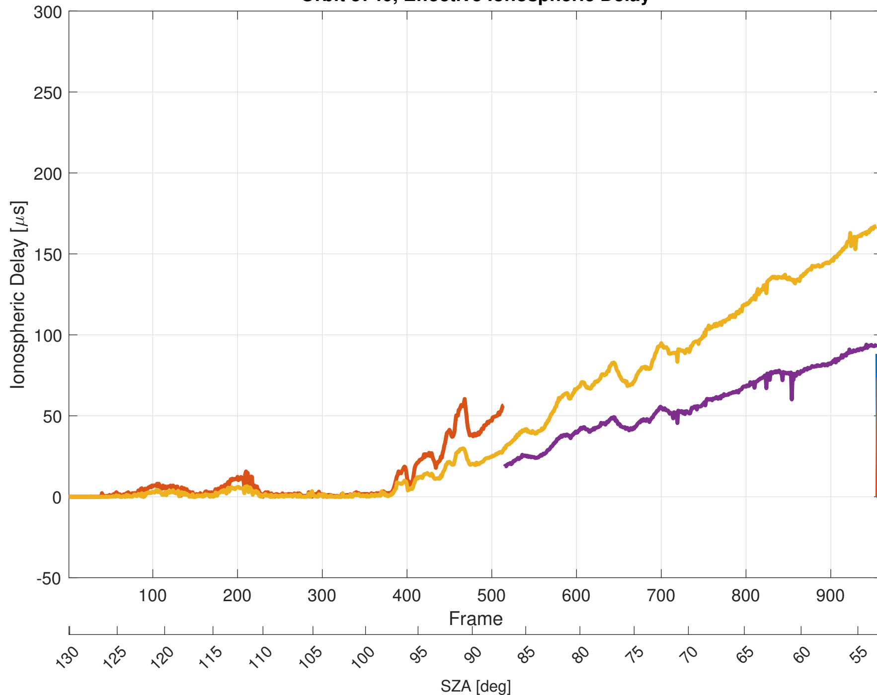
Orbit 5740, Effective Ionospheric Delay
