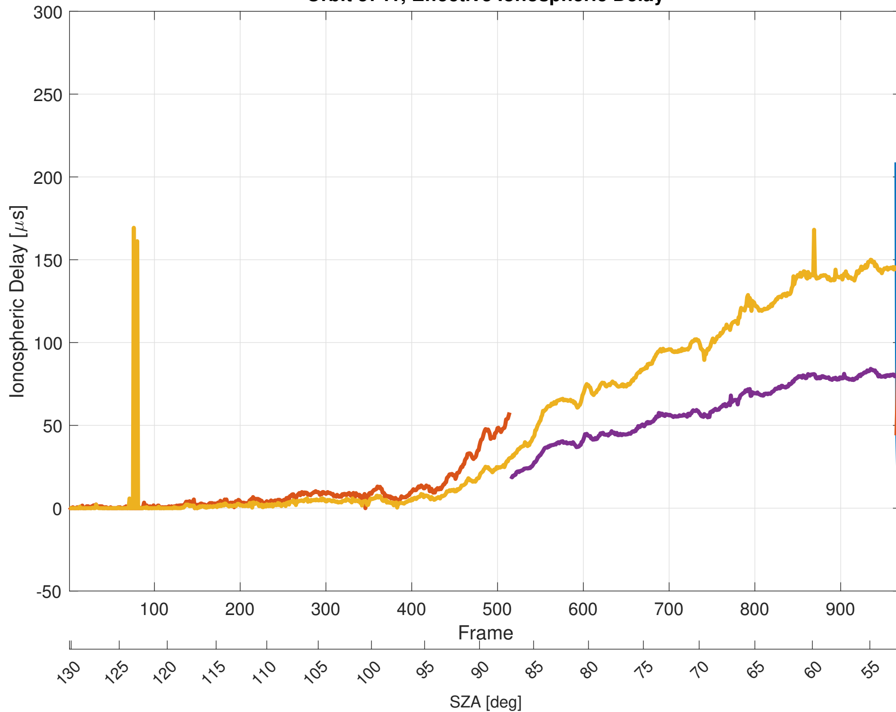
Orbit 5741, Effective Ionospheric Delay
