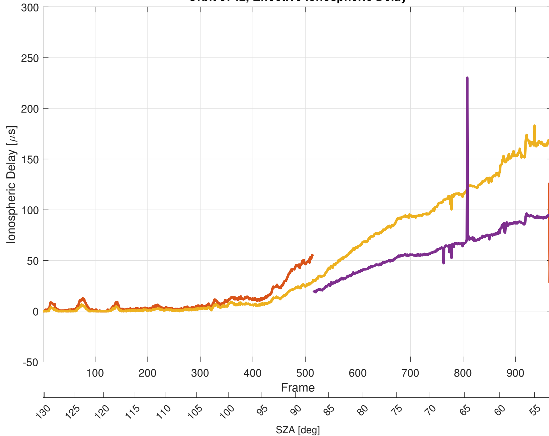
Orbit 5742, Effective Ionospheric Delay
