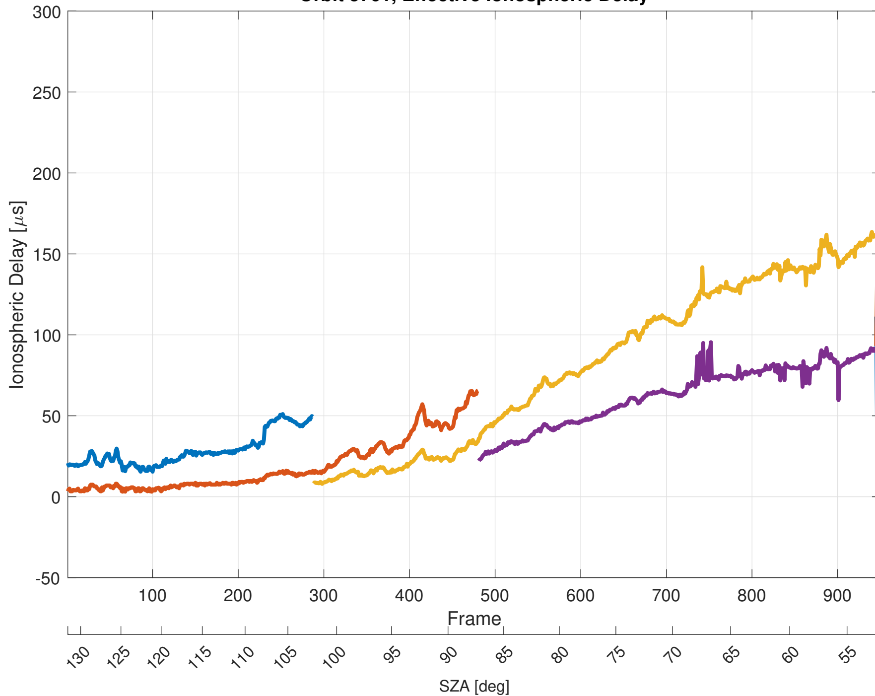
Orbit 5761, Effective Ionospheric Delay
