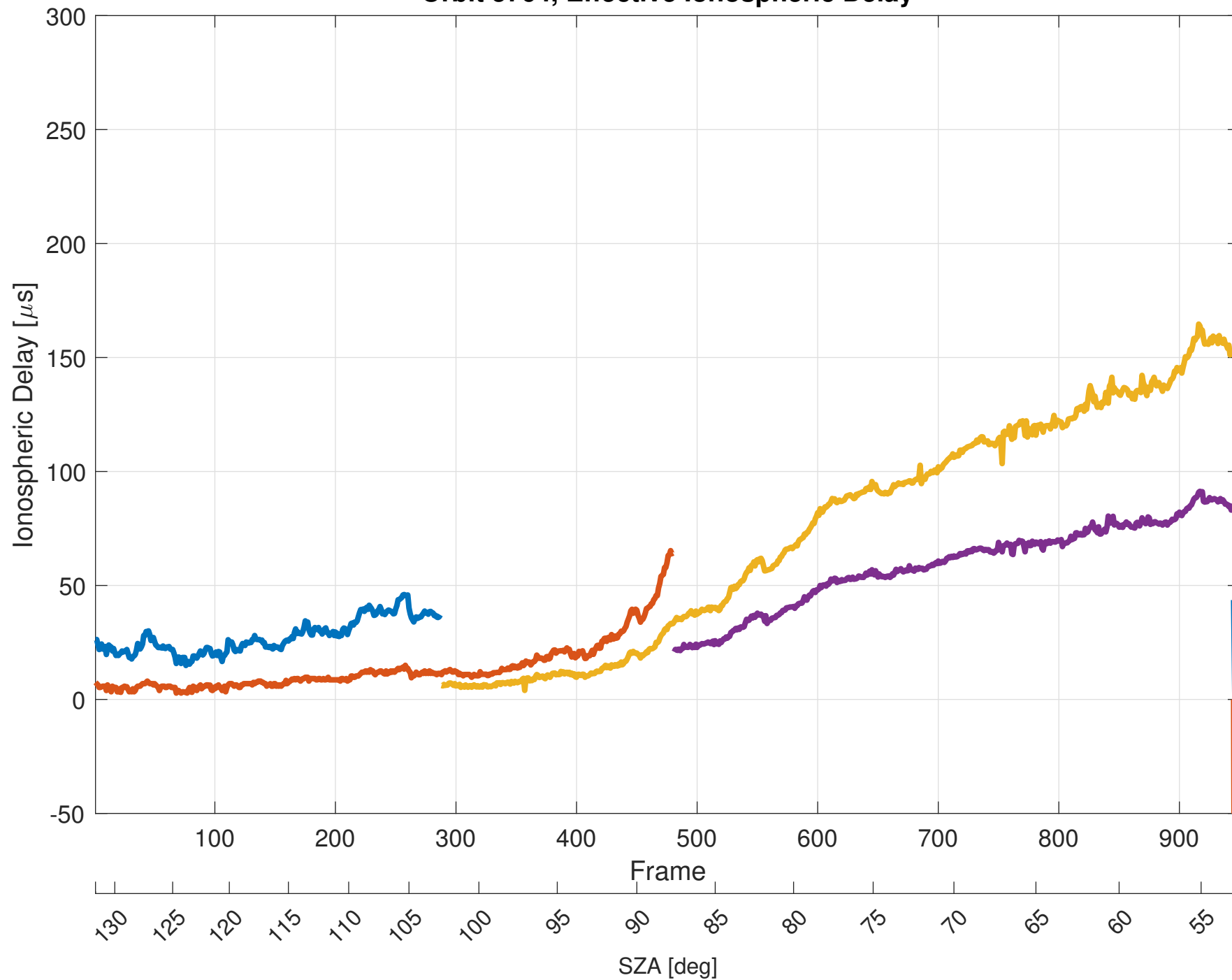
Orbit 5764, Effective Ionospheric Delay
