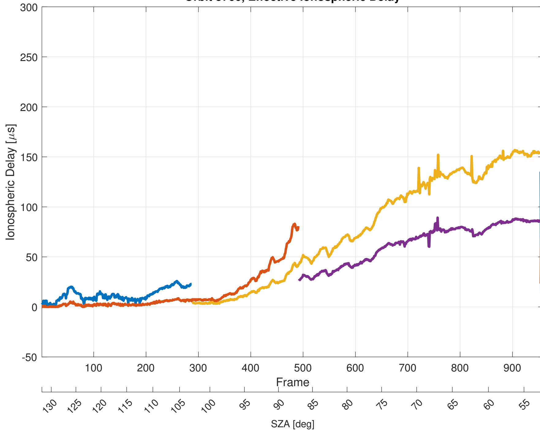
Orbit 5766, Effective Ionospheric Delay
