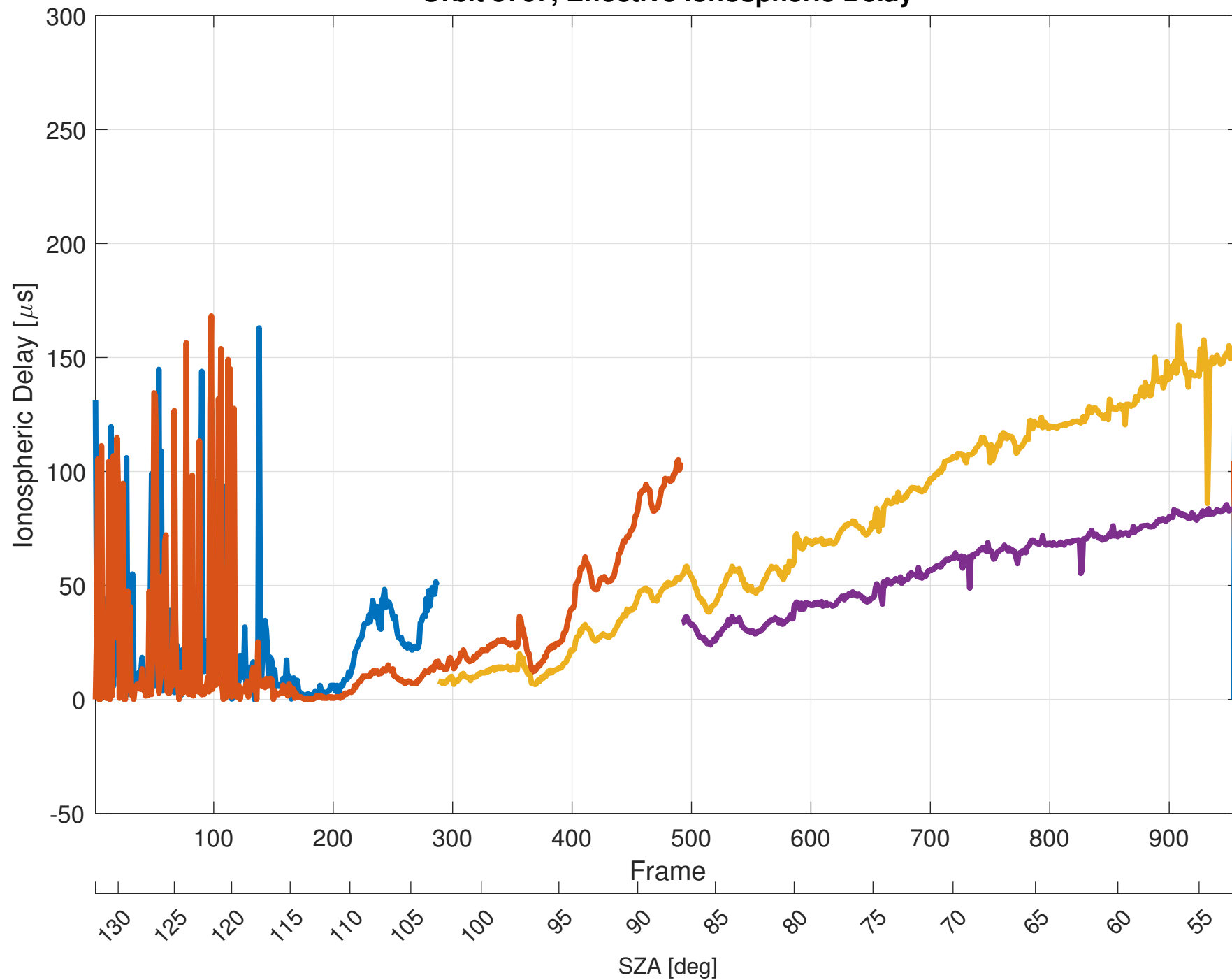
Orbit 5767, Effective Ionospheric Delay
