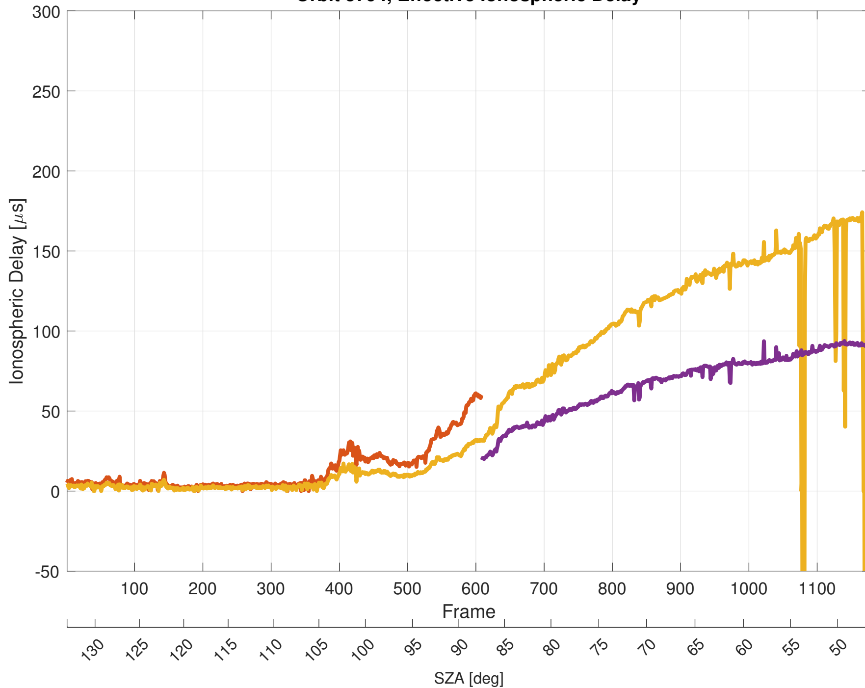
Orbit 5794, Effective Ionospheric Delay
