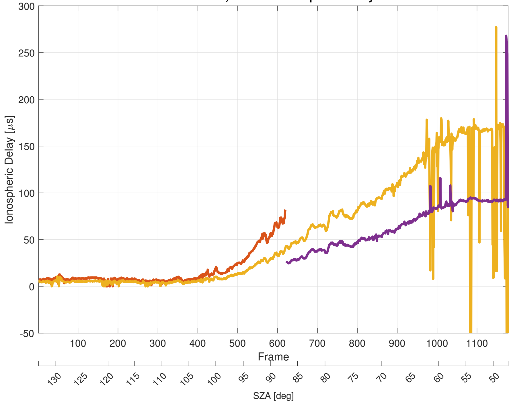
Orbit 5799, Effective Ionospheric Delay
