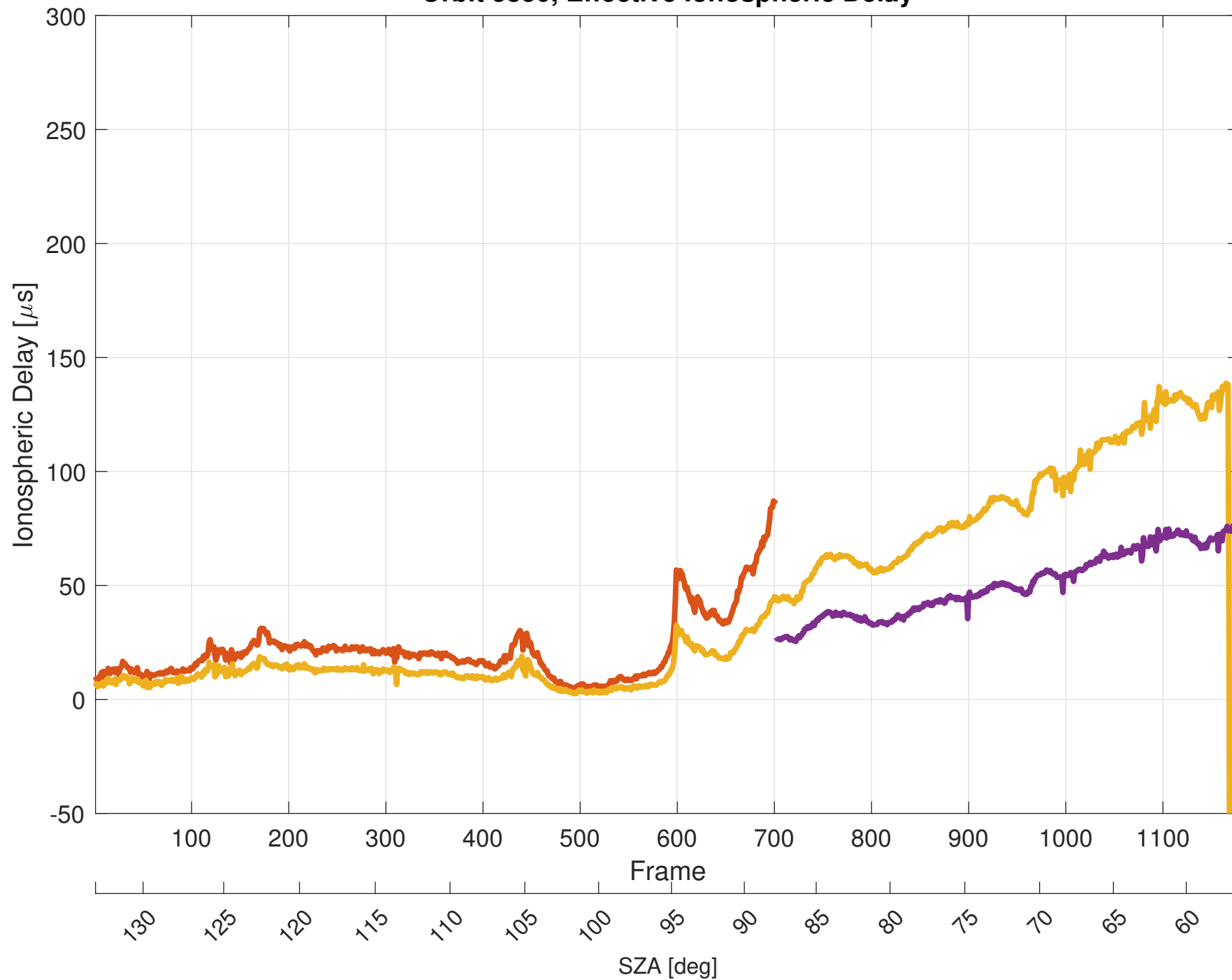
Orbit 5850, Effective Ionospheric Delay
