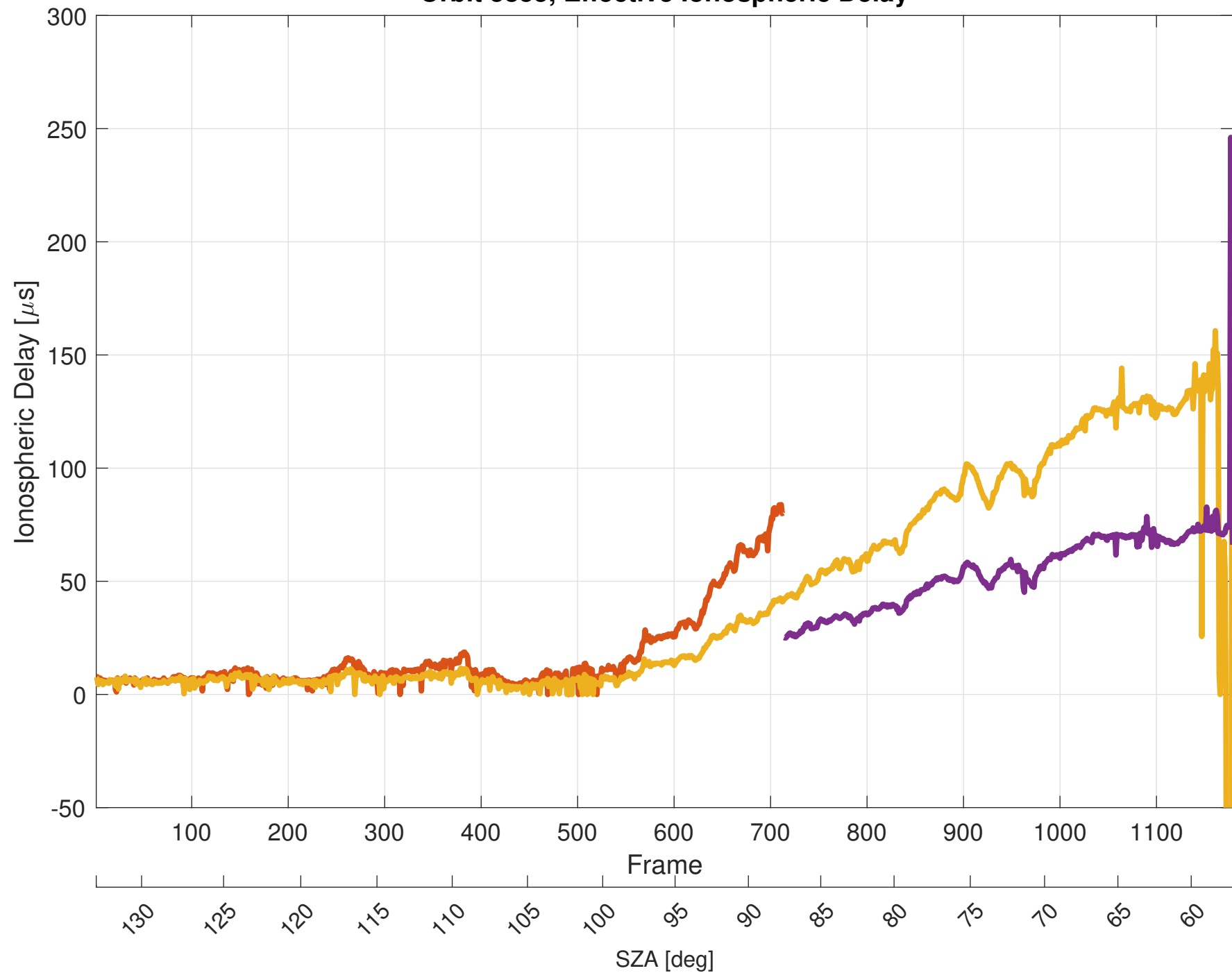
Orbit 5855, Effective Ionospheric Delay
