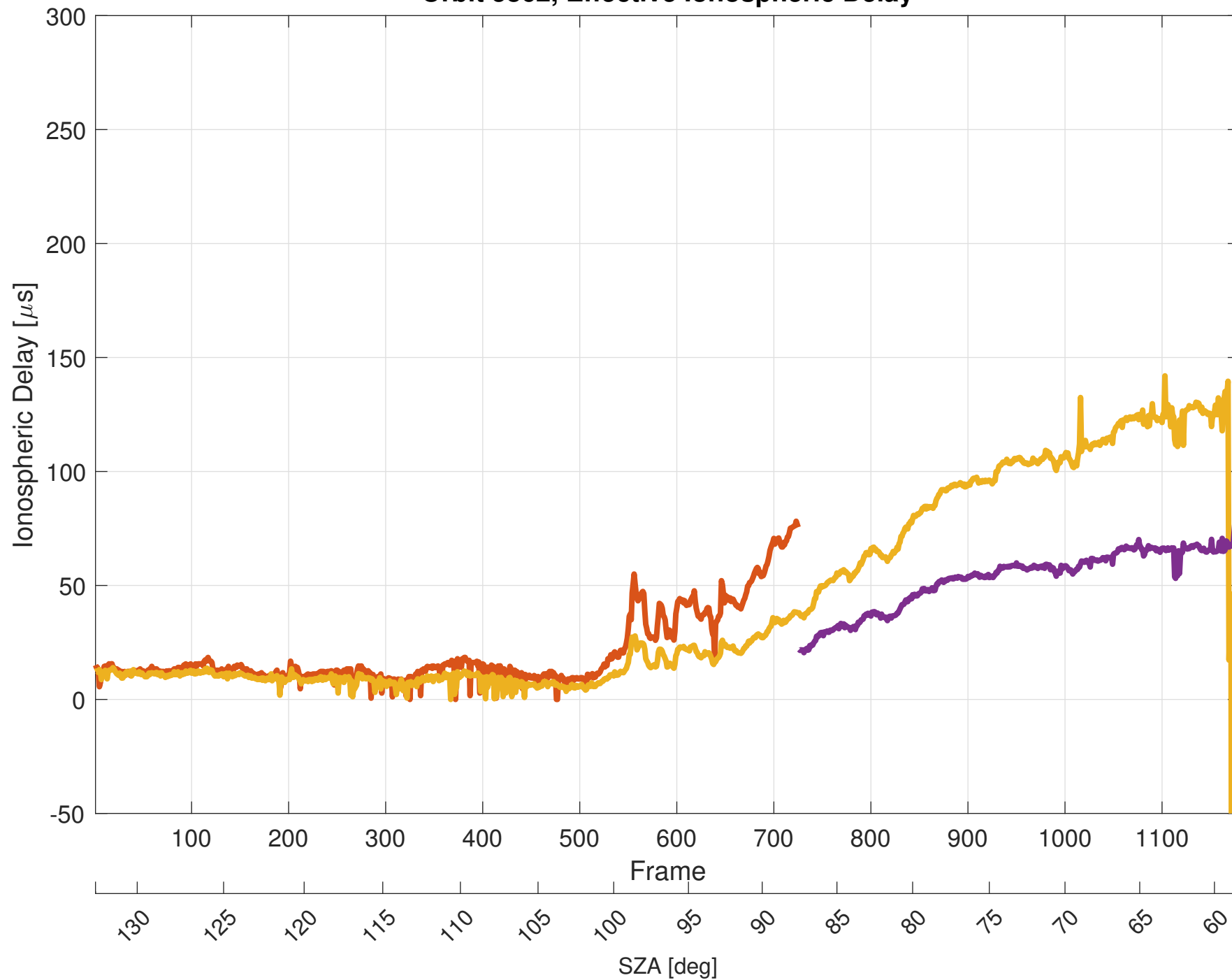
Orbit 5862, Effective Ionospheric Delay
