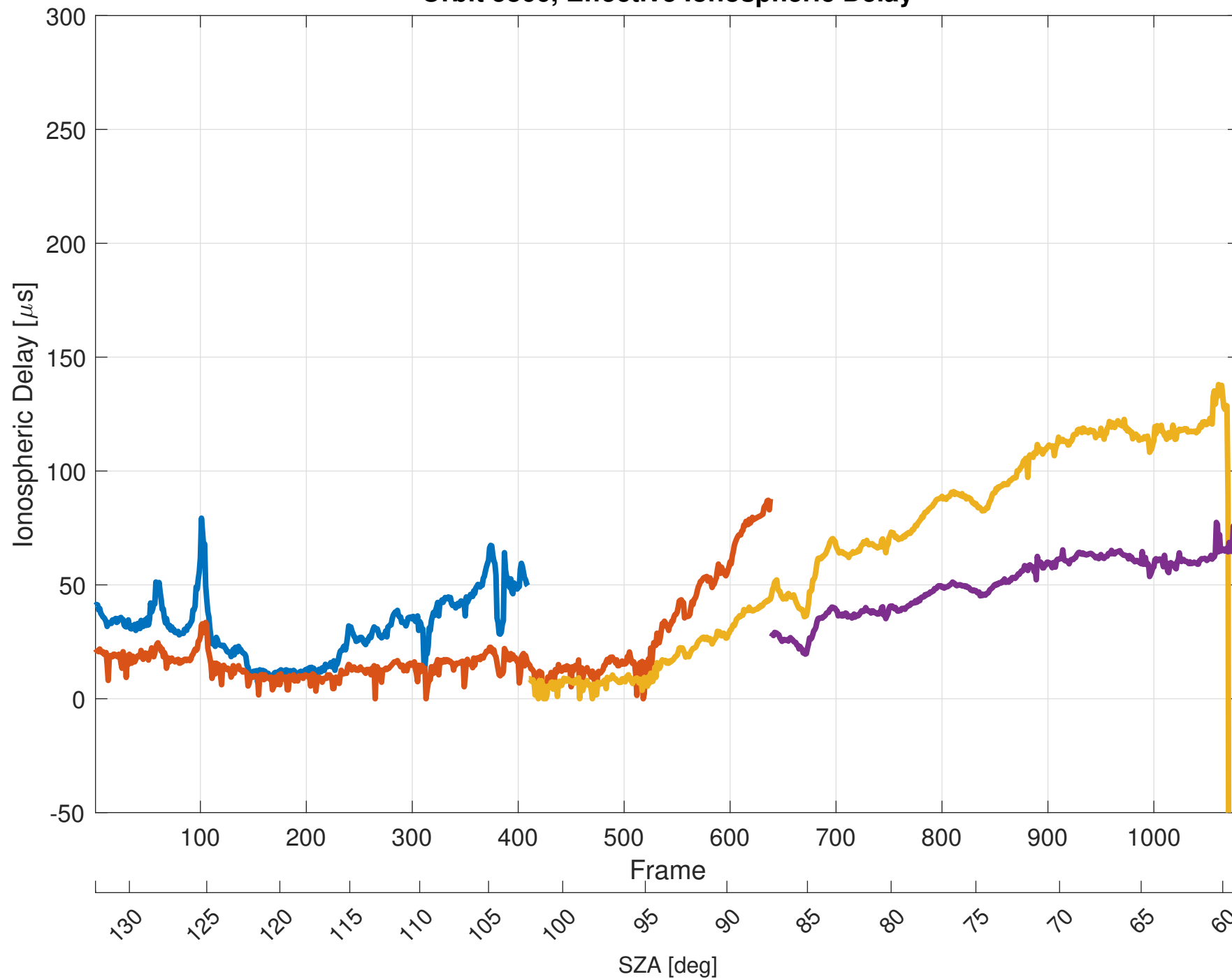
Orbit 5866, Effective Ionospheric Delay
