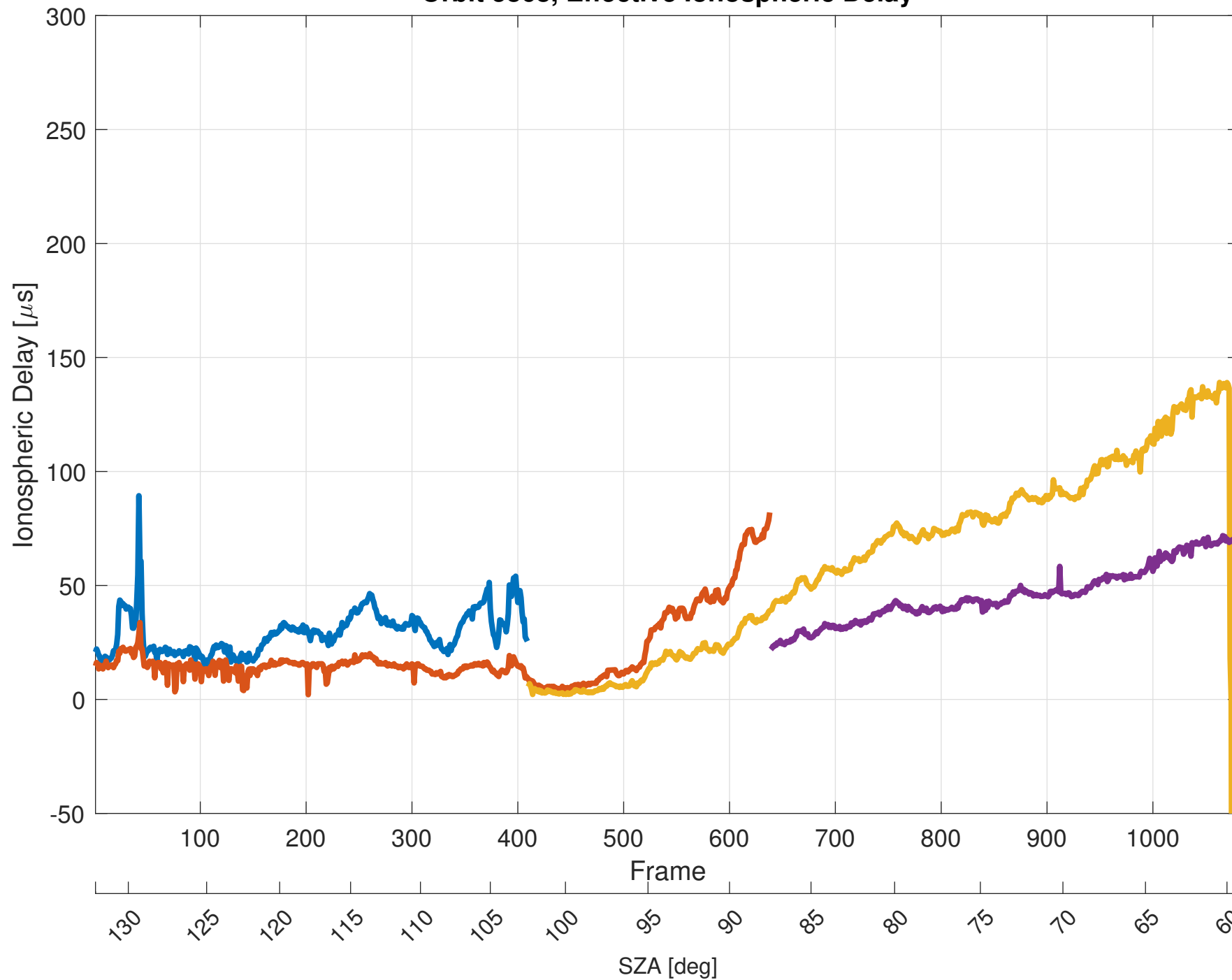
Orbit 5868, Effective Ionospheric Delay
