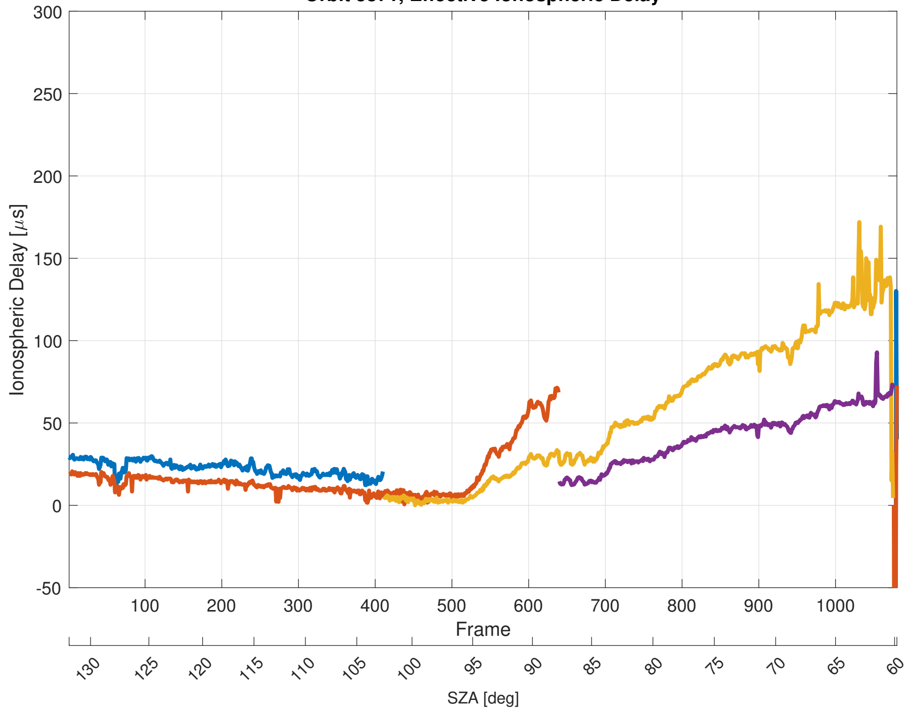
Orbit 5871, Effective Ionospheric Delay
