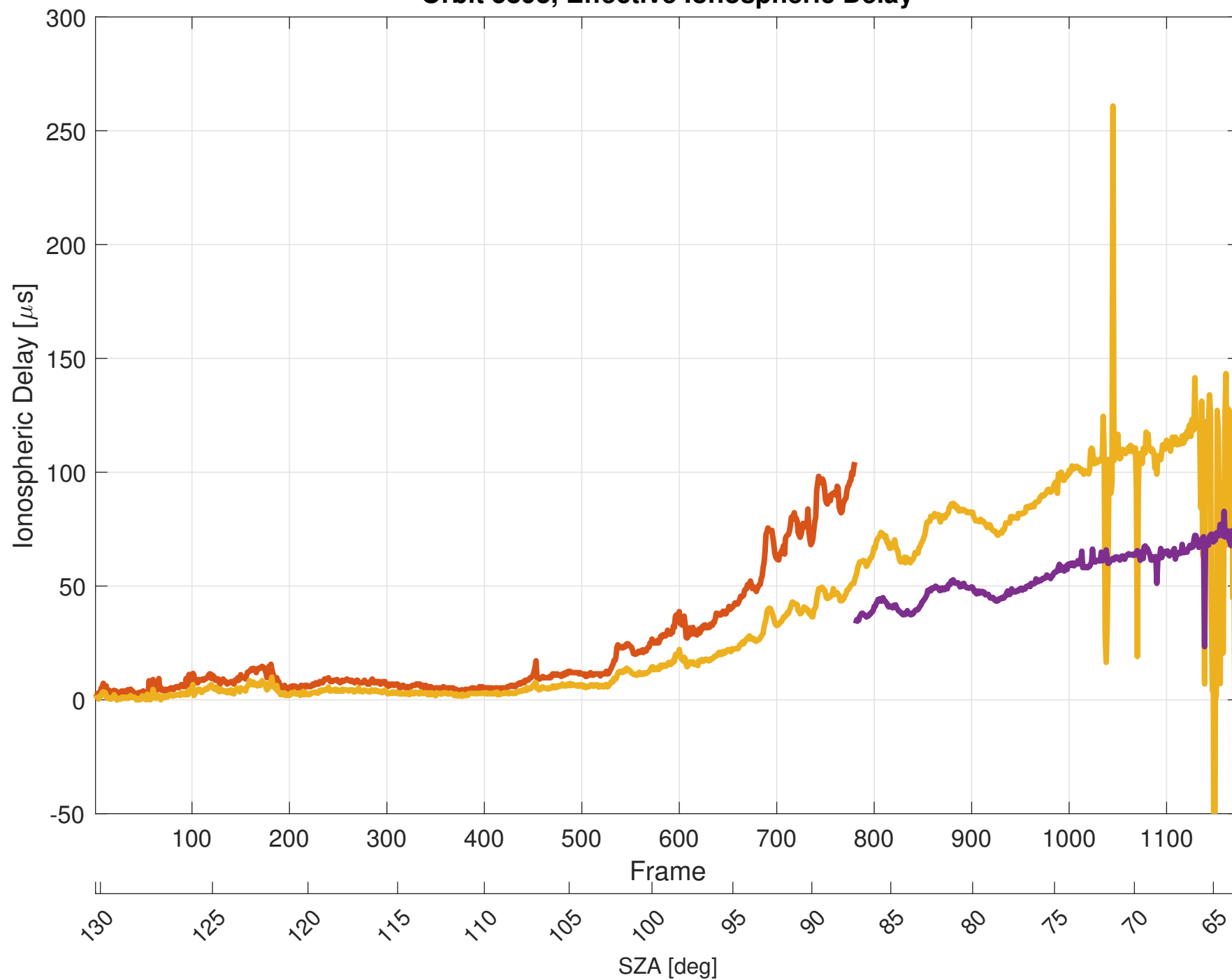
Orbit 5893, Effective Ionospheric Delay
