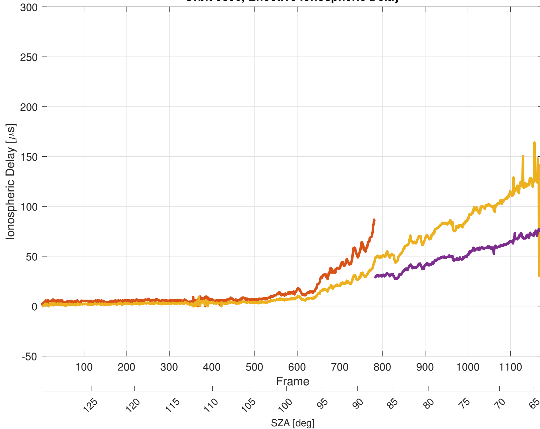
Orbit 5896, Effective Ionospheric Delay
