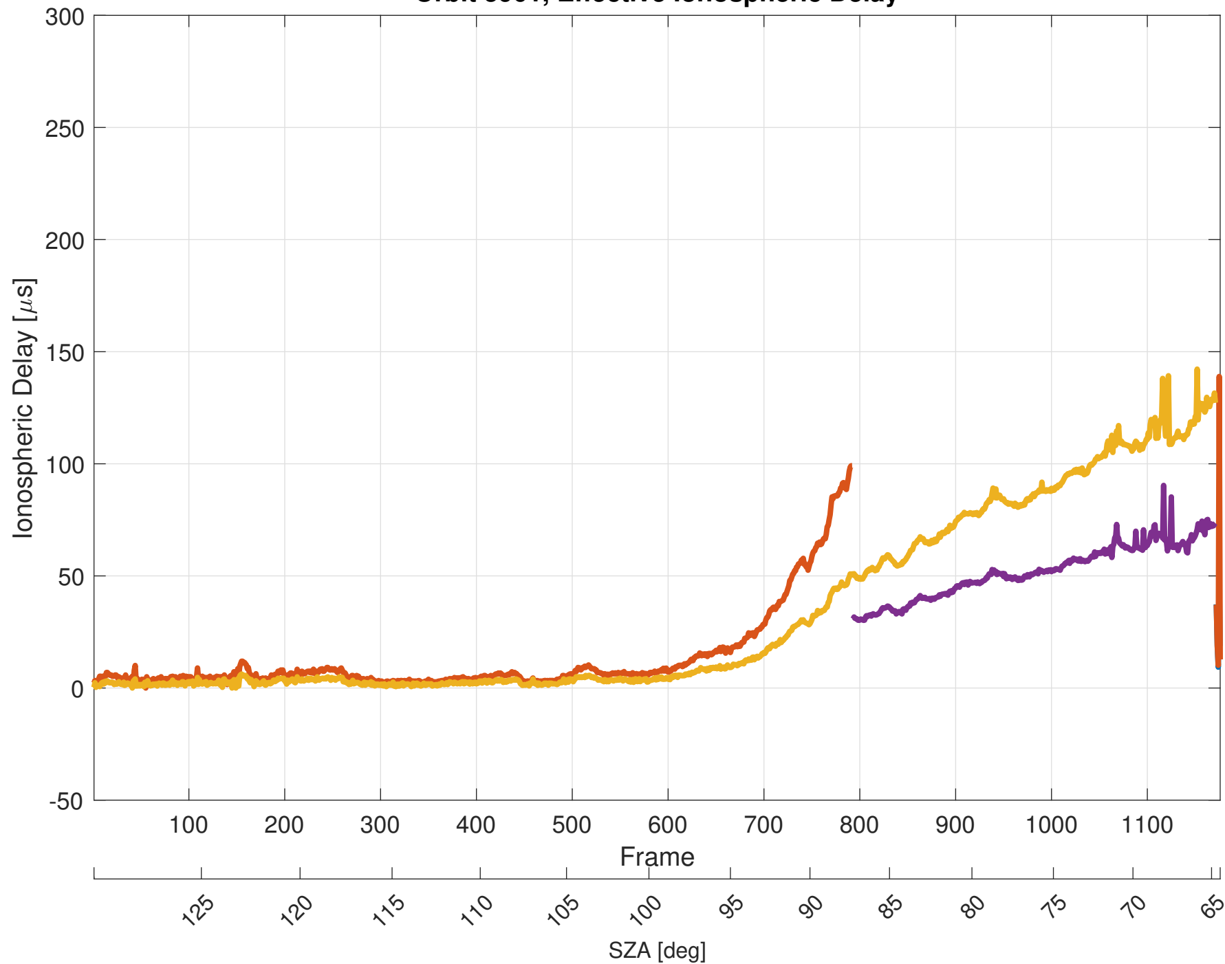
Orbit 5901, Effective Ionospheric Delay
