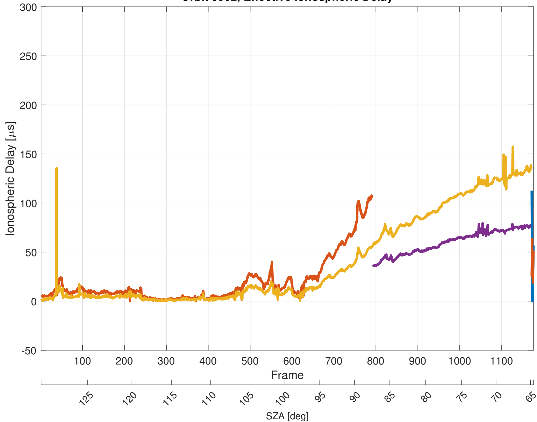
Orbit 5902, Effective Ionospheric Delay
