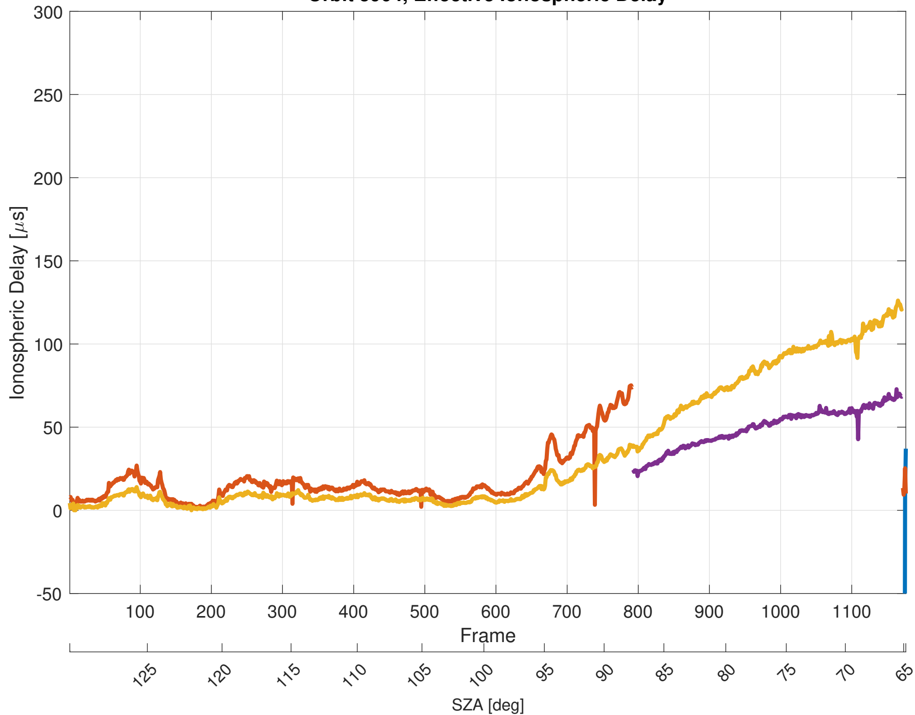
Orbit 5904, Effective Ionospheric Delay
