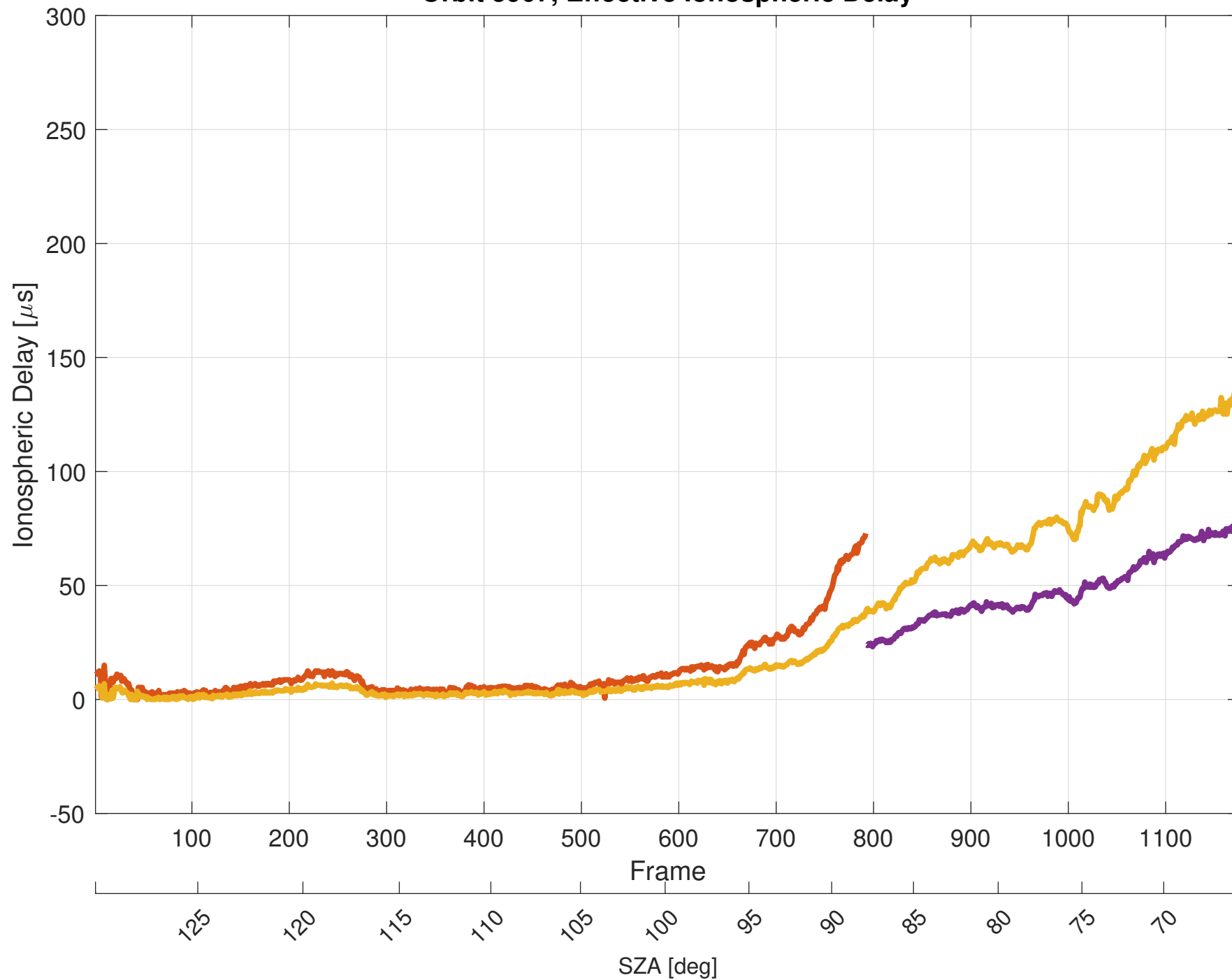
Orbit 5907, Effective Ionospheric Delay
