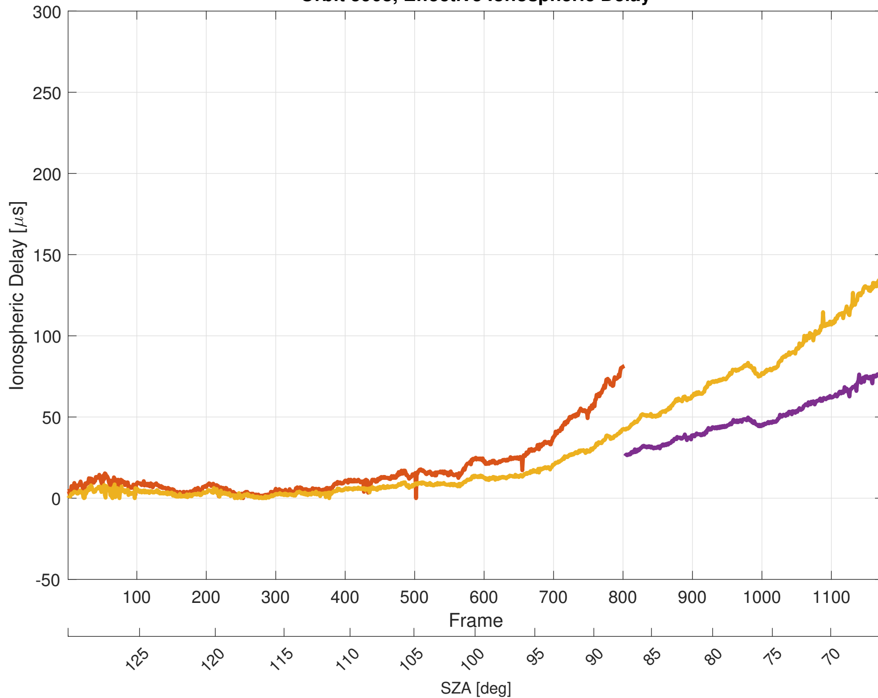
Orbit 5908, Effective Ionospheric Delay
