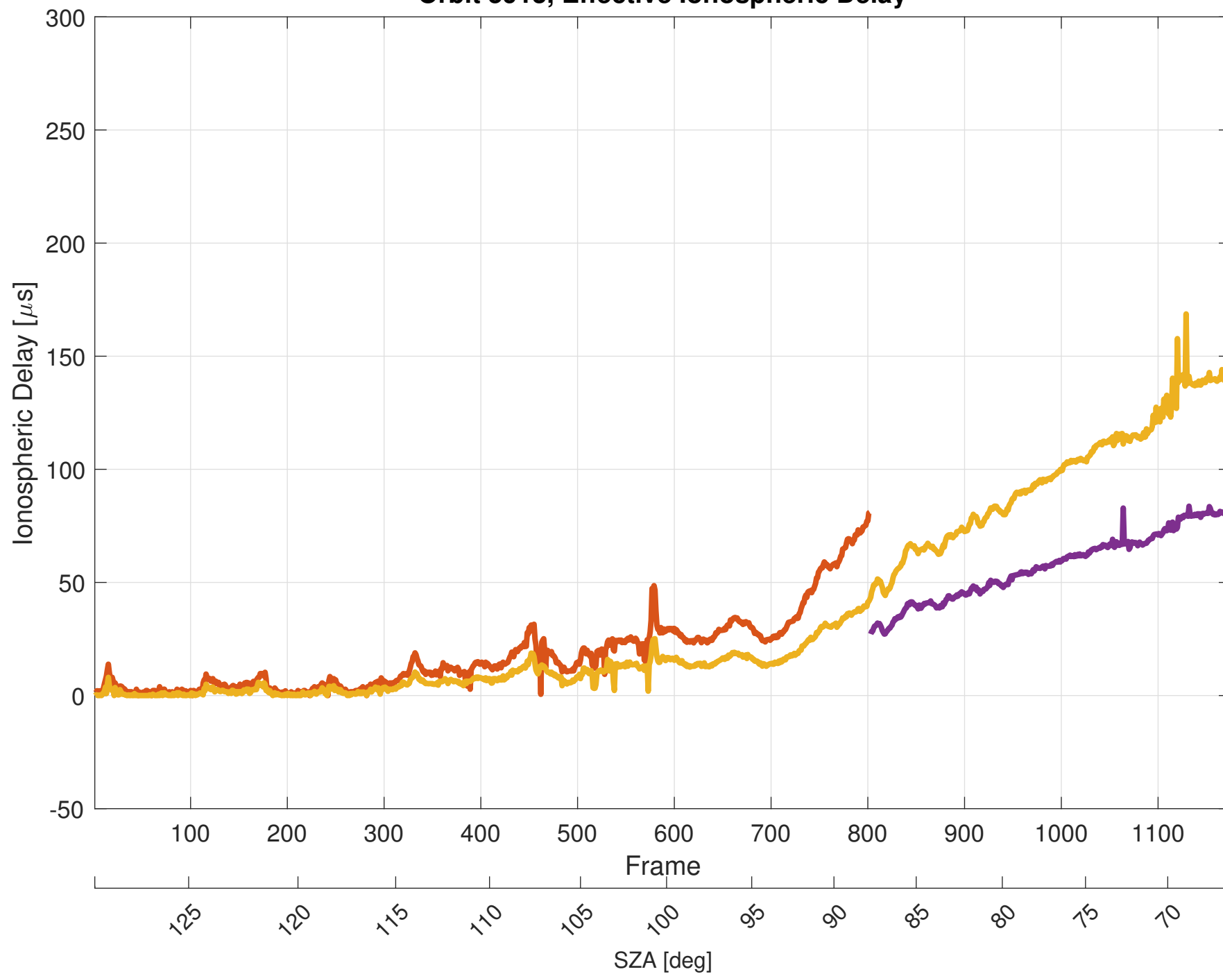
Orbit 5913, Effective Ionospheric Delay
