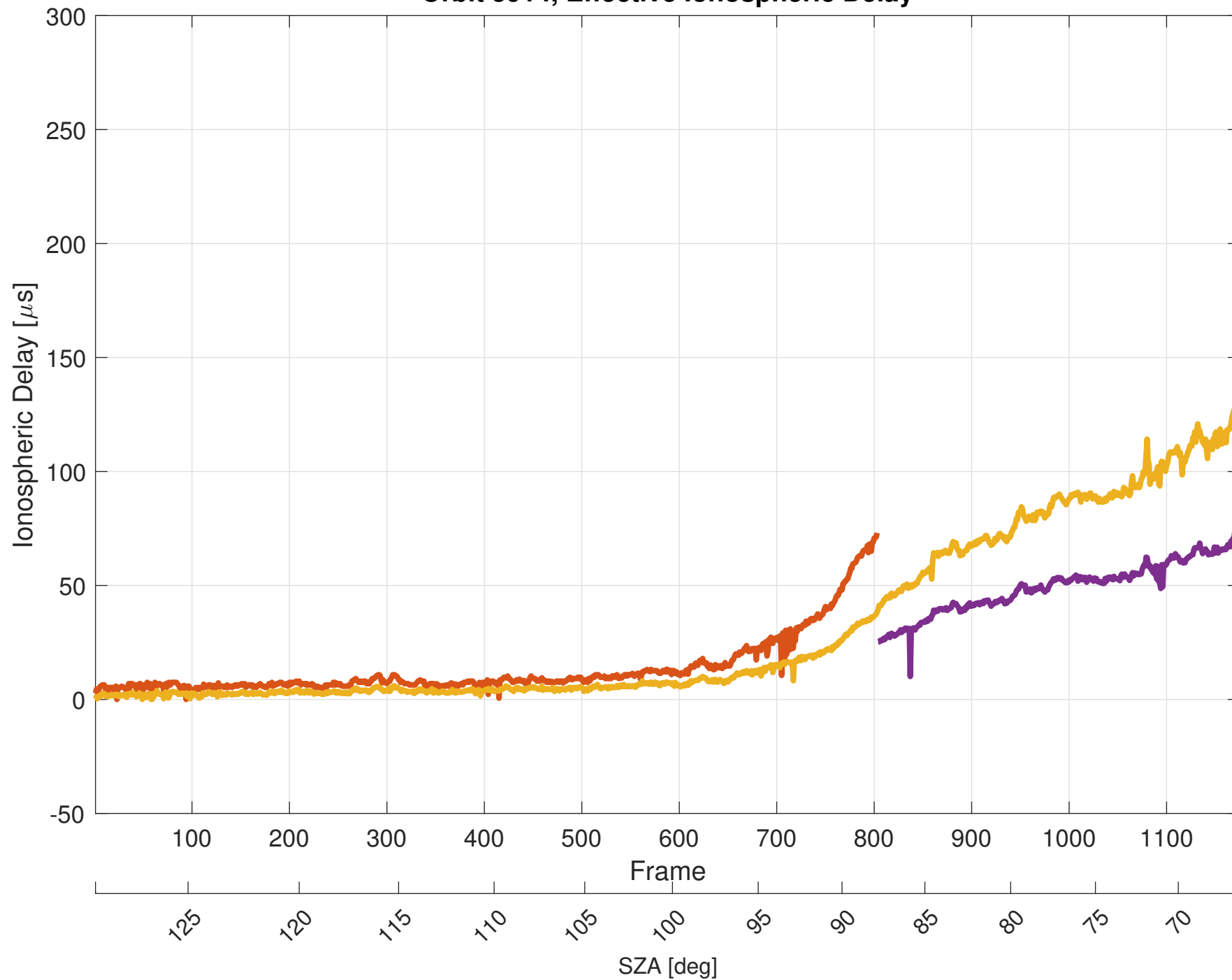
Orbit 5914, Effective Ionospheric Delay
