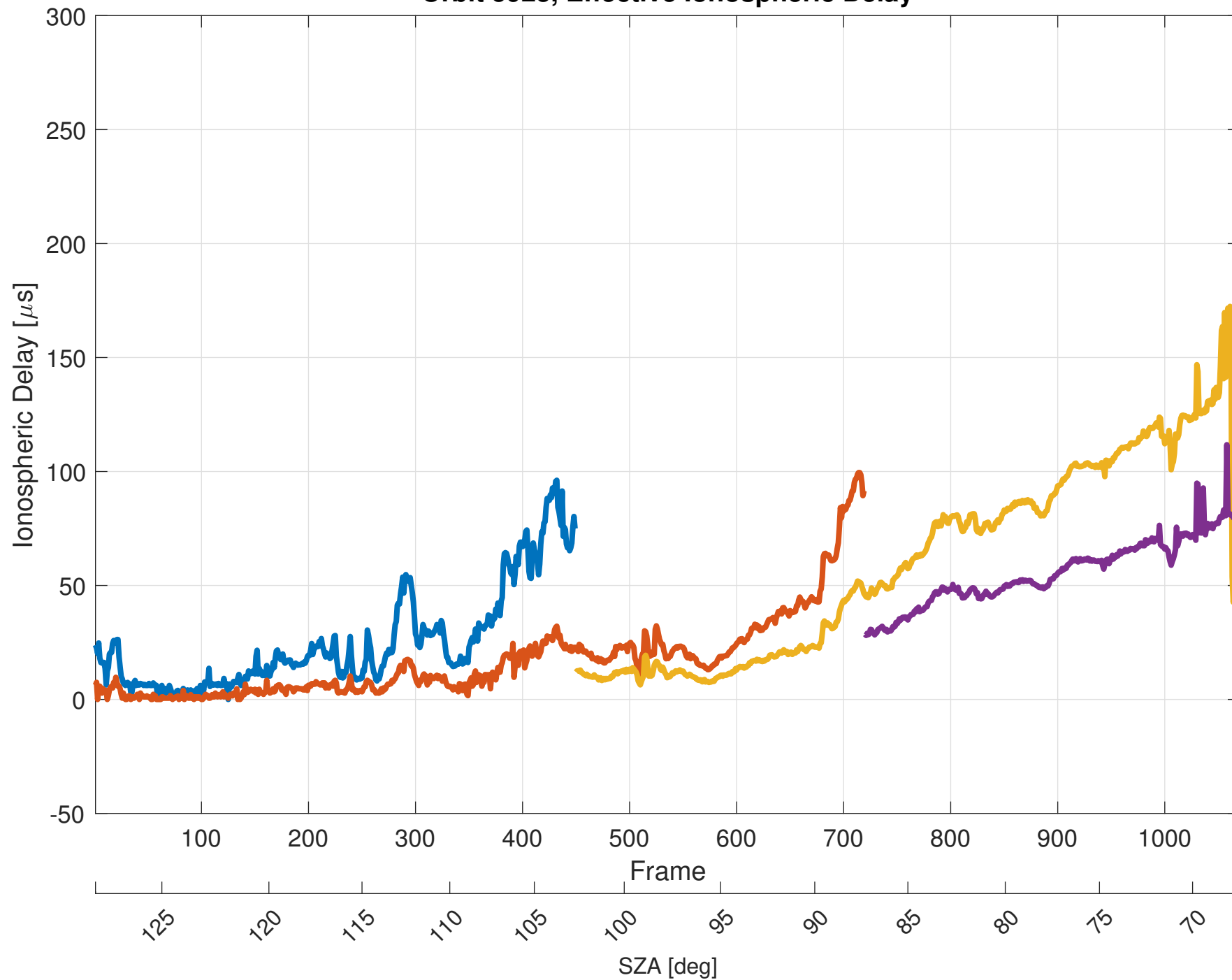
Orbit 5923, Effective Ionospheric Delay
