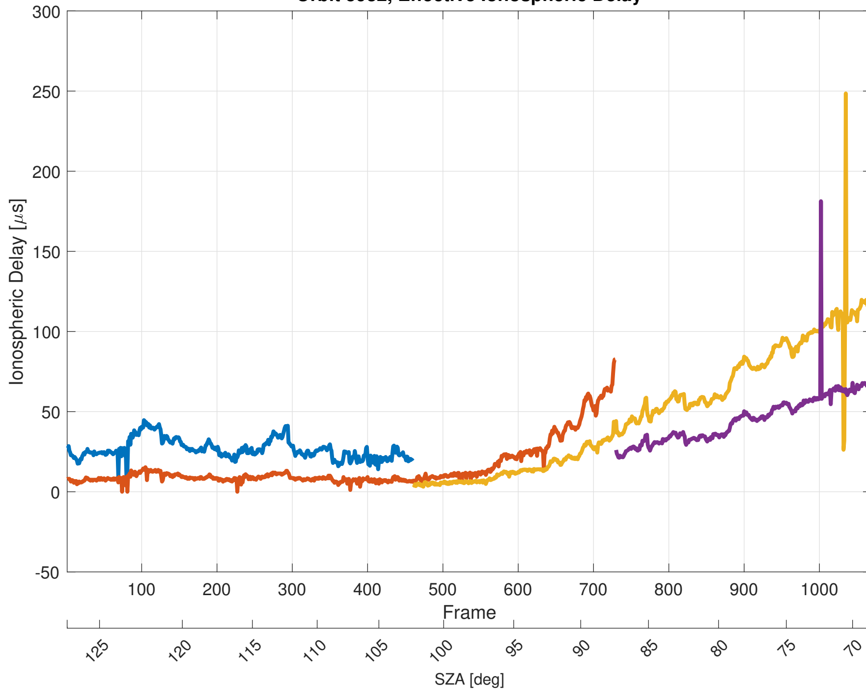
Orbit 5932, Effective Ionospheric Delay
