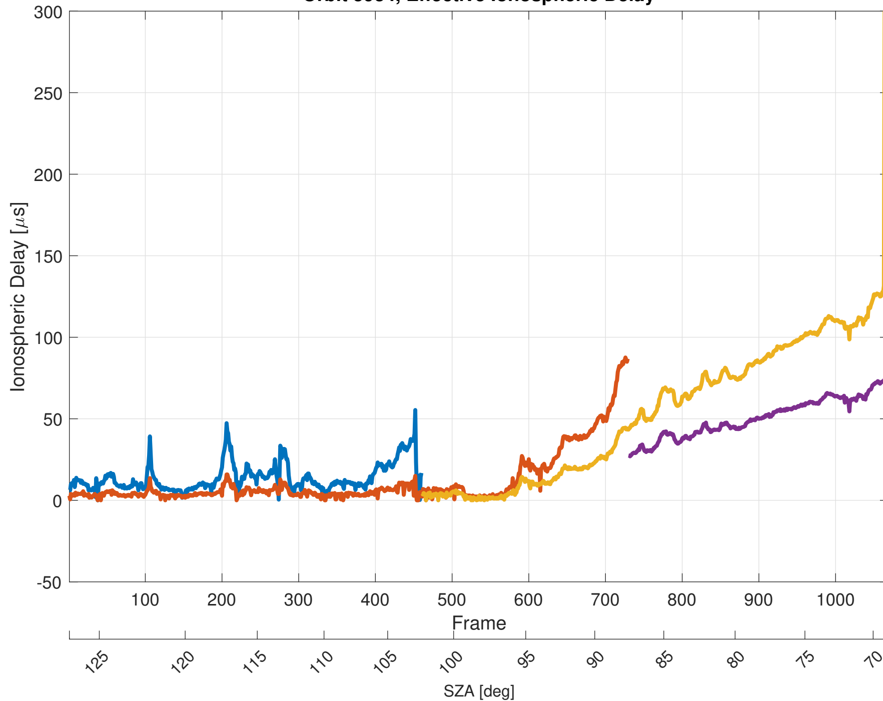
Orbit 5934, Effective Ionospheric Delay
