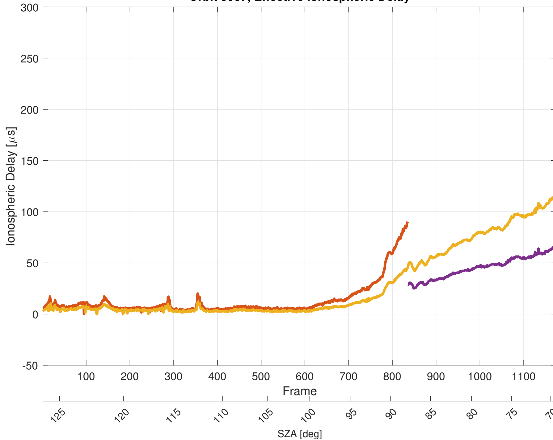
Orbit 5937, Effective Ionospheric Delay
