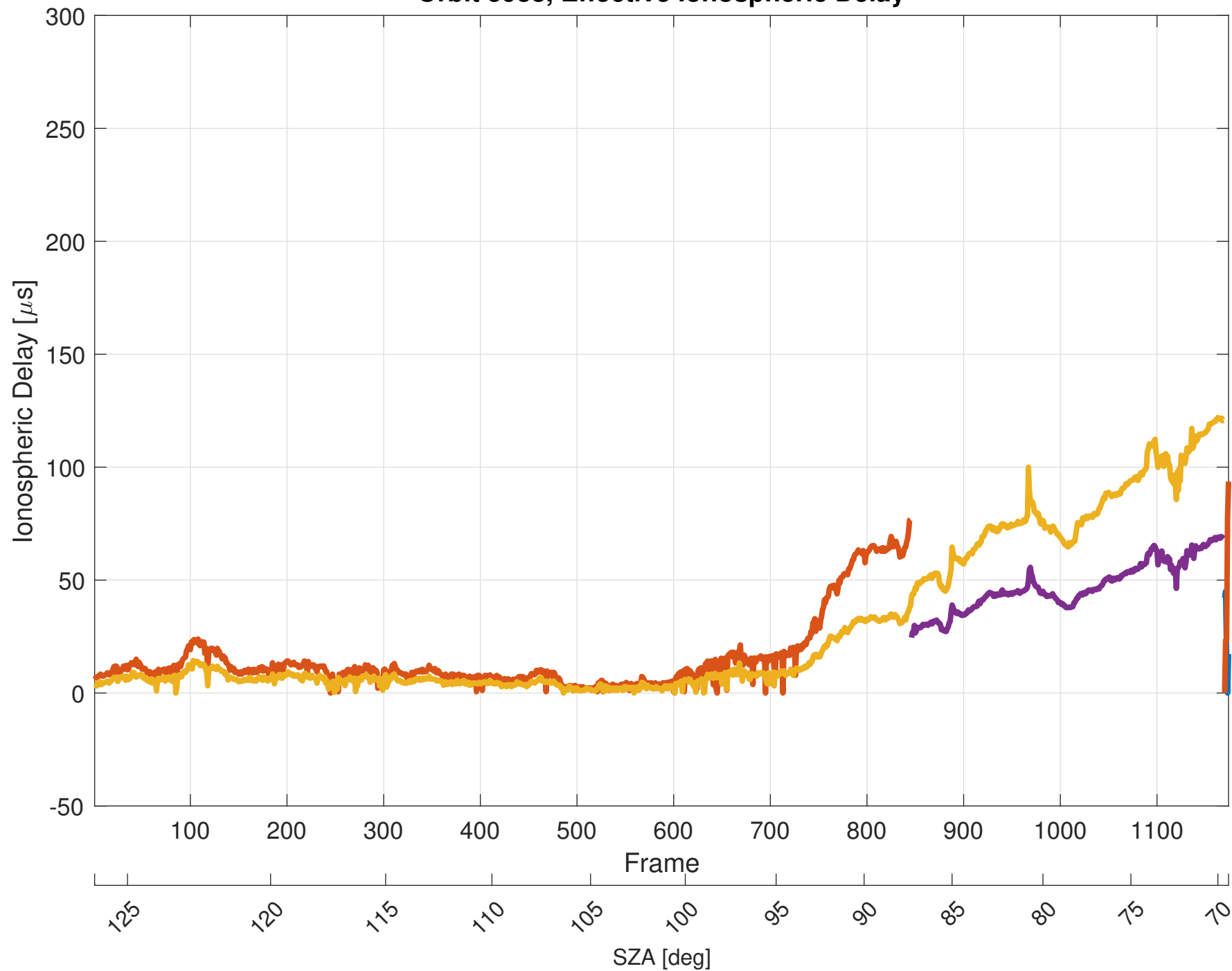
Orbit 5938, Effective Ionospheric Delay
