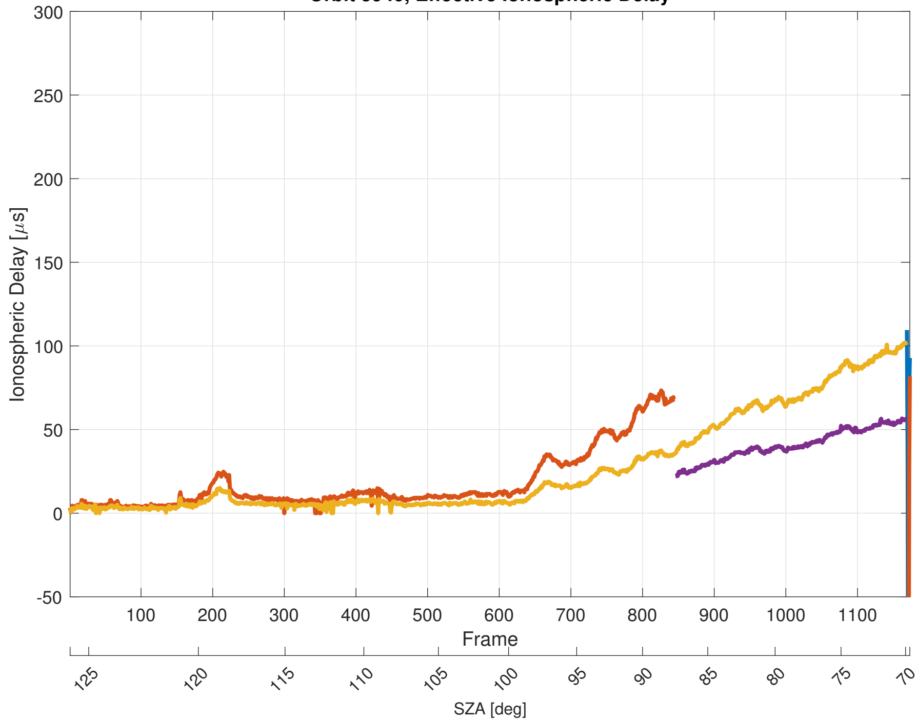
Orbit 5940, Effective Ionospheric Delay
