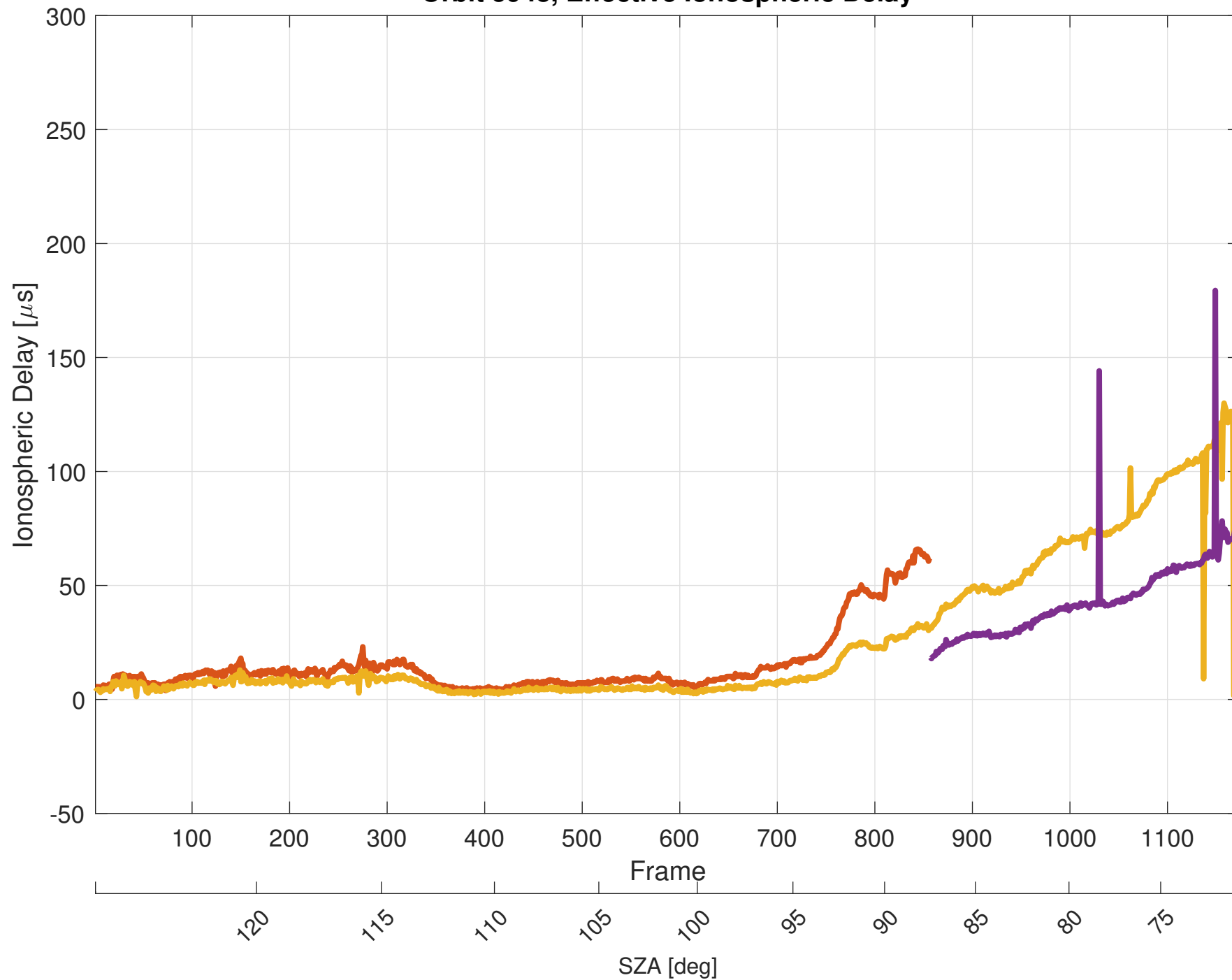
Orbit 5948, Effective Ionospheric Delay
