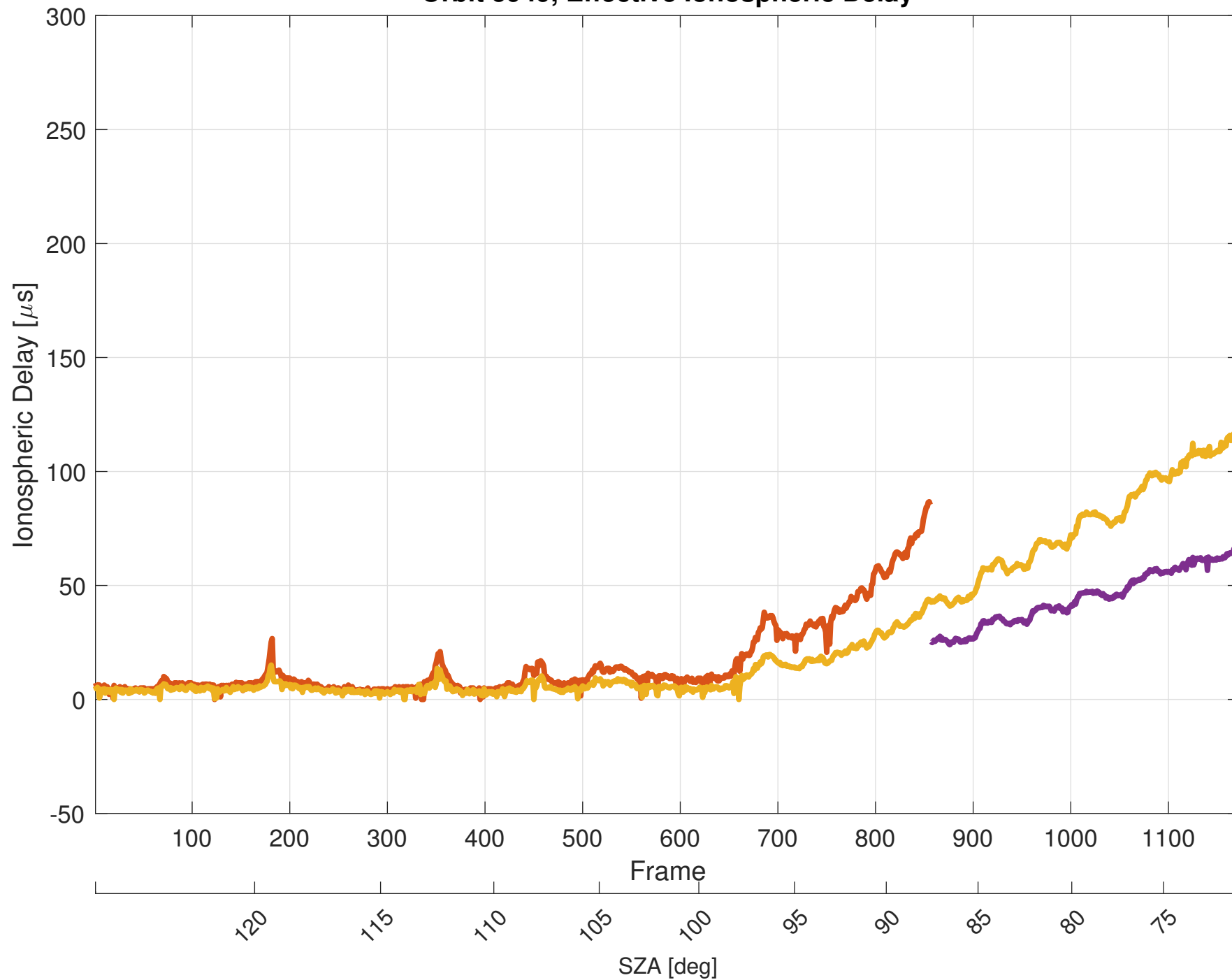
Orbit 5949, Effective Ionospheric Delay
