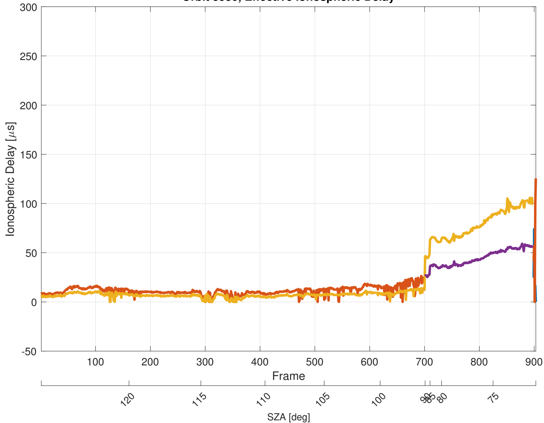
Orbit 5950, Effective Ionospheric Delay
