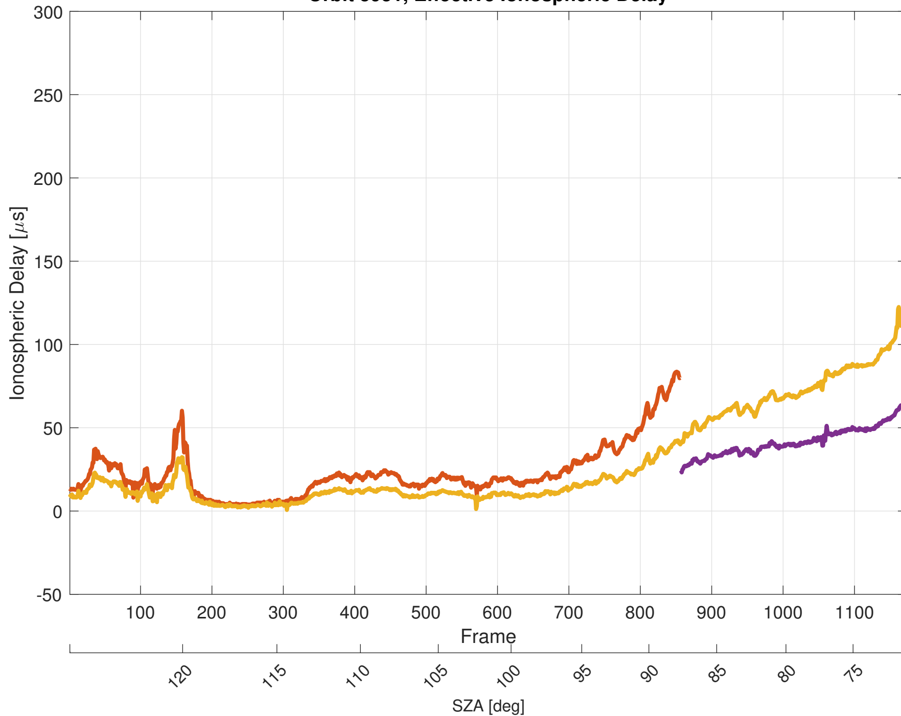
Orbit 5951, Effective Ionospheric Delay
