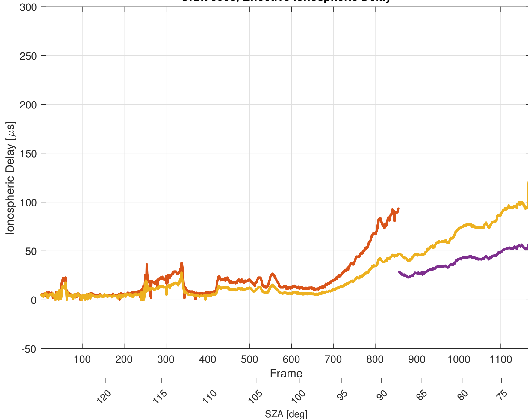
Orbit 5953, Effective Ionospheric Delay
