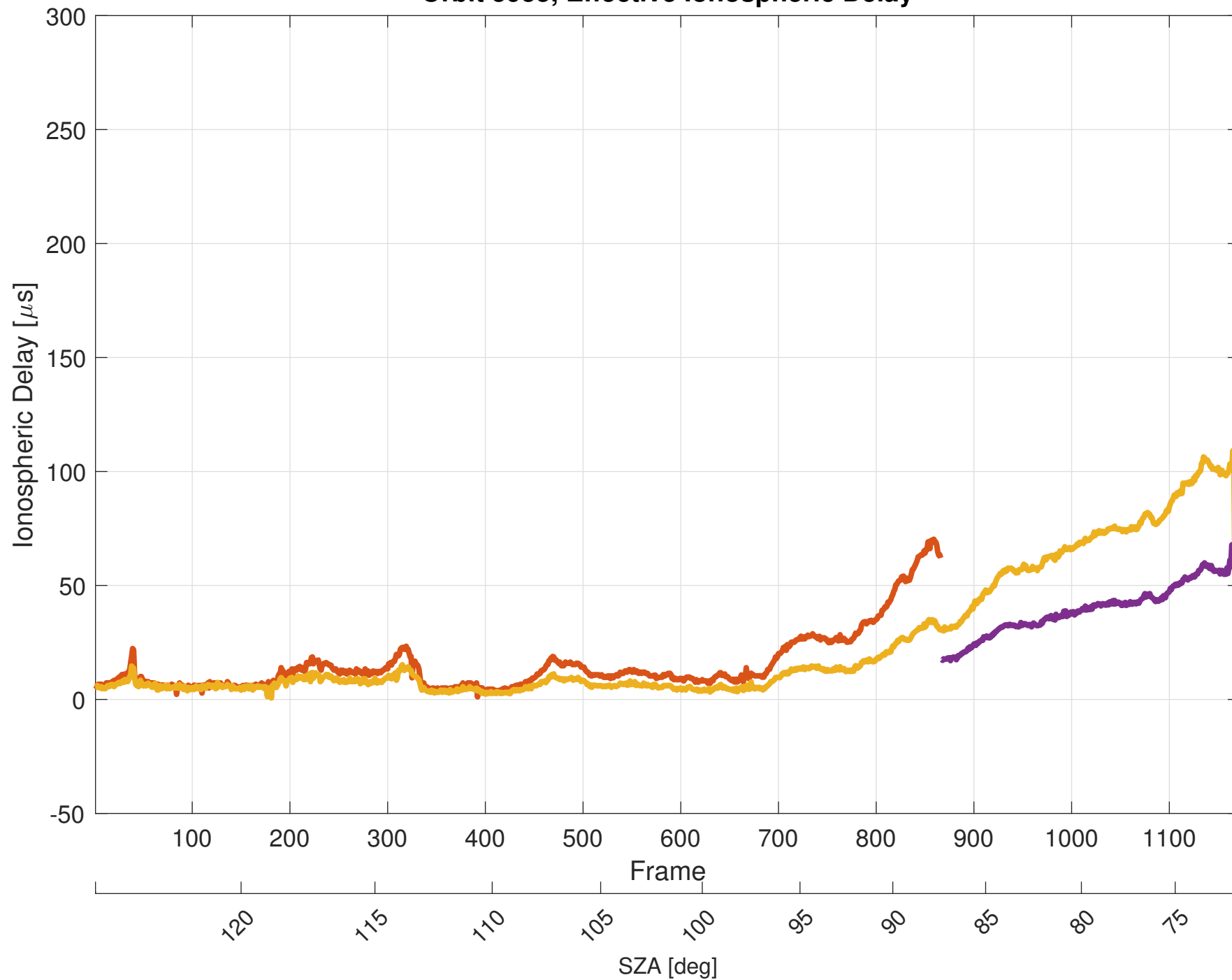
Orbit 5955, Effective Ionospheric Delay
