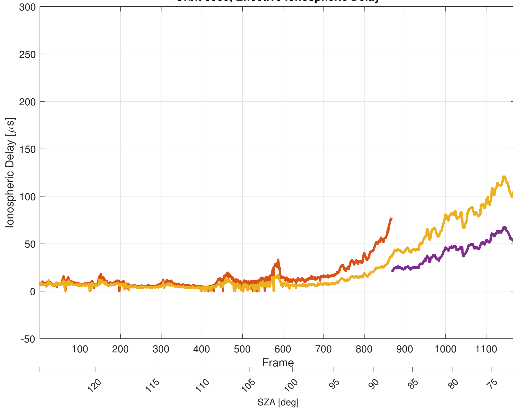
Orbit 5959, Effective Ionospheric Delay
