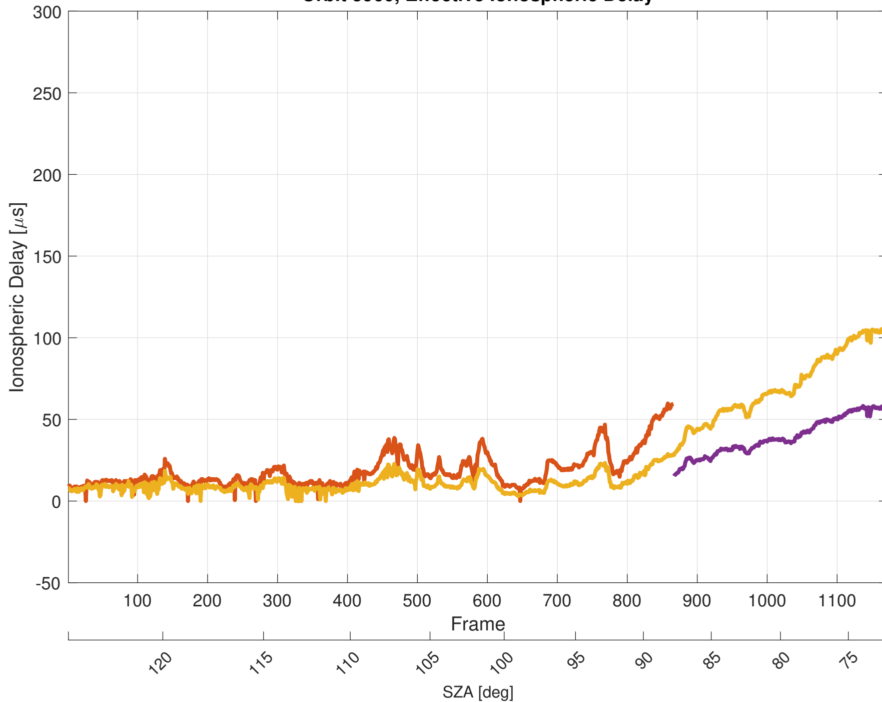
Orbit 5960, Effective Ionospheric Delay
