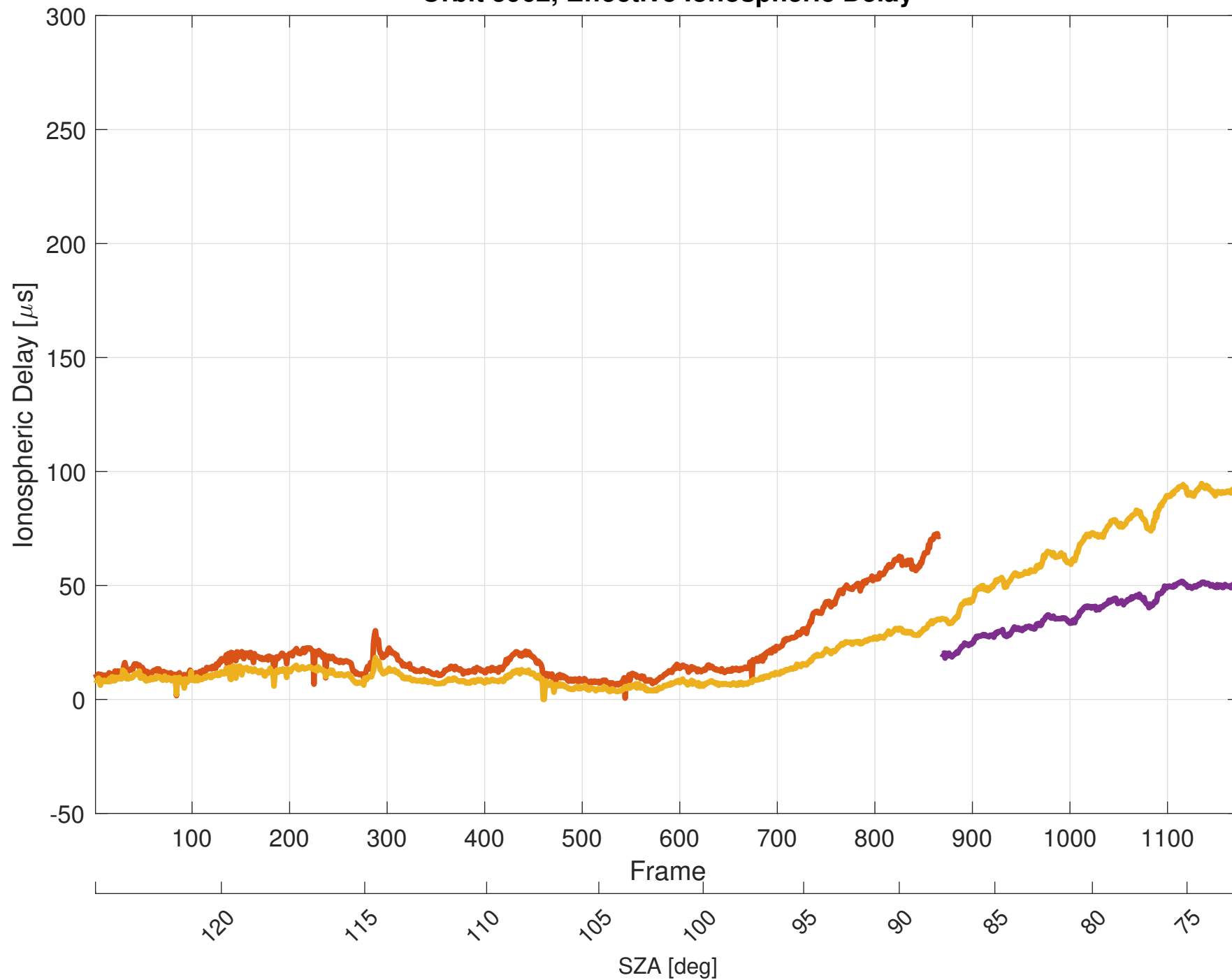
Orbit 5962, Effective Ionospheric Delay
