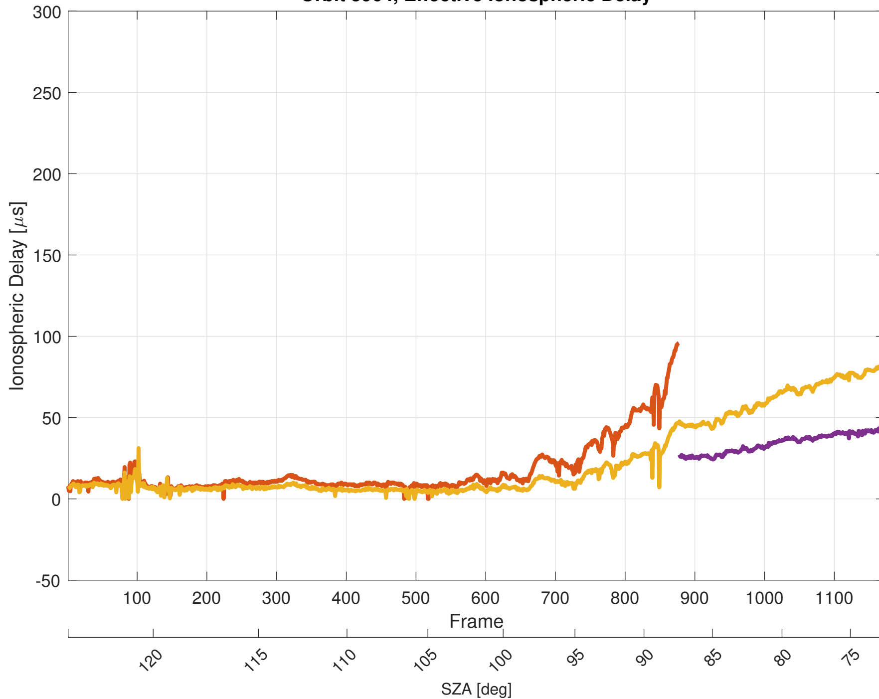
Orbit 5964, Effective Ionospheric Delay
