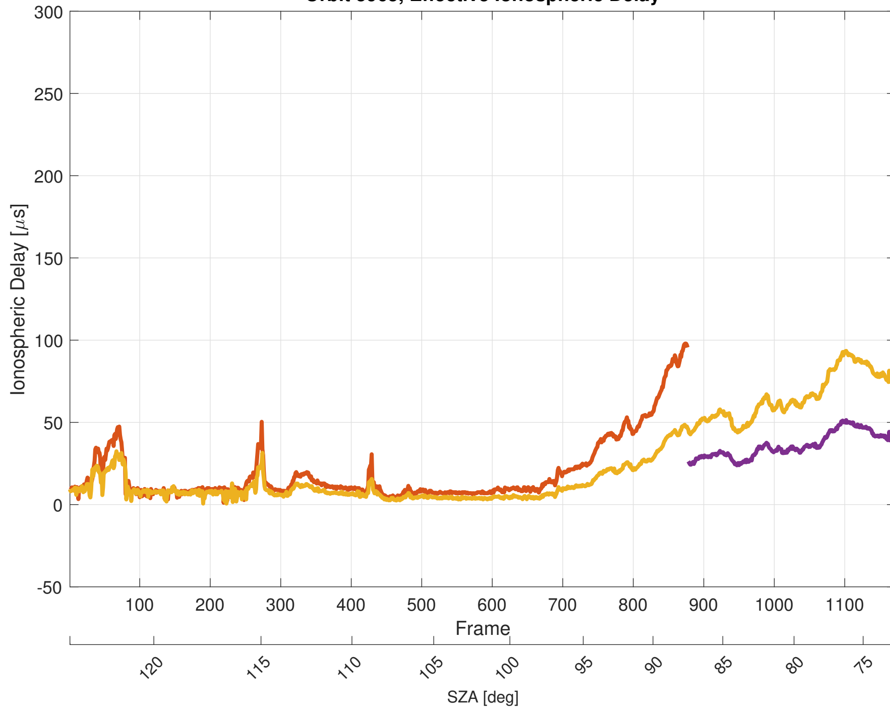
Orbit 5965, Effective Ionospheric Delay
