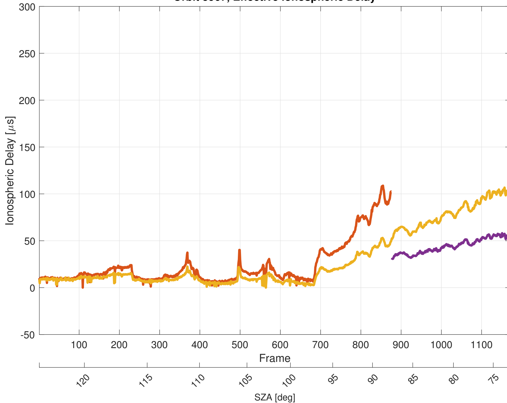
Orbit 5967, Effective Ionospheric Delay
