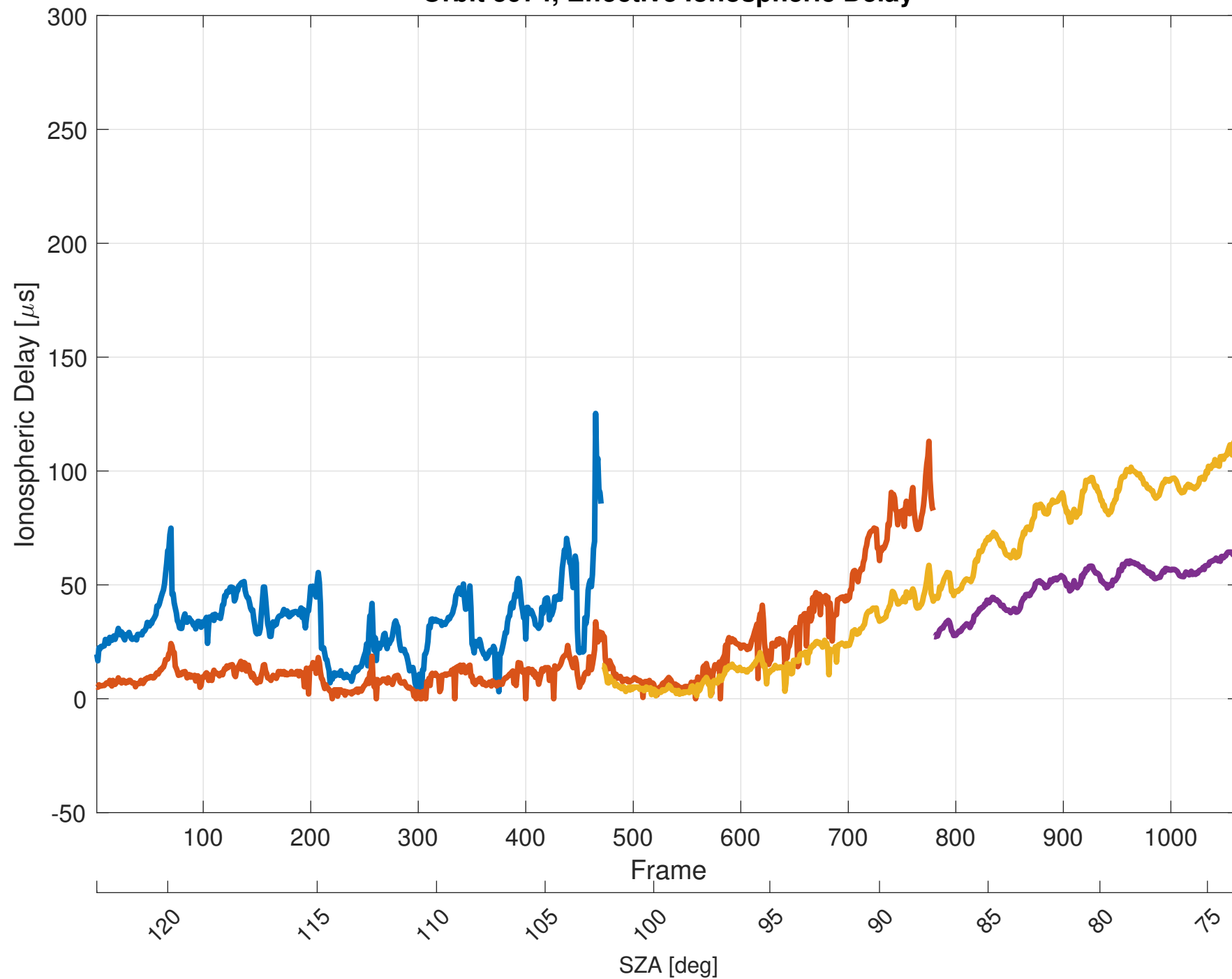
Orbit 5974, Effective Ionospheric Delay
