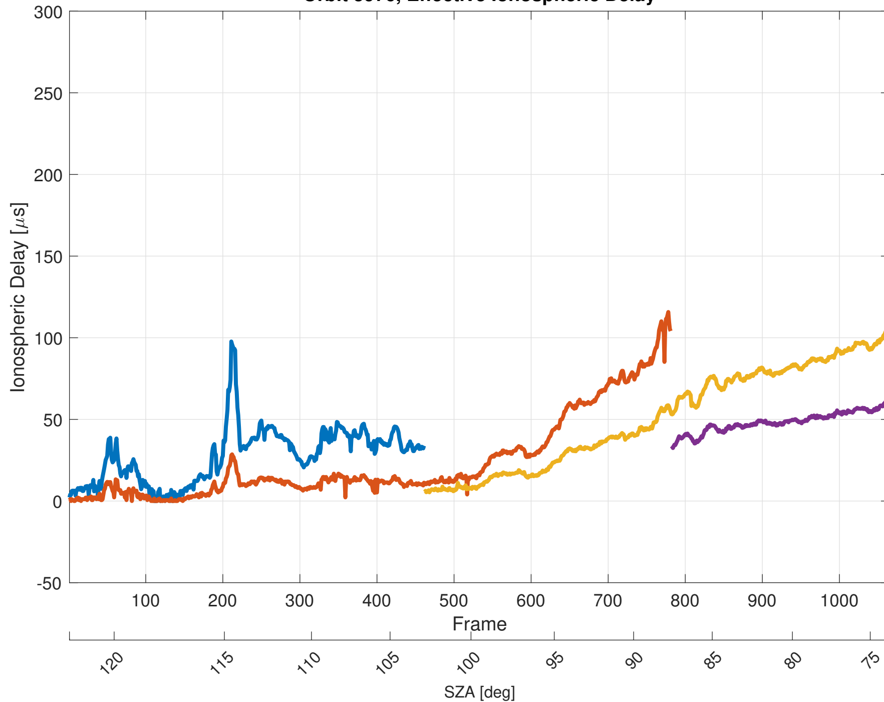
Orbit 5976, Effective Ionospheric Delay
