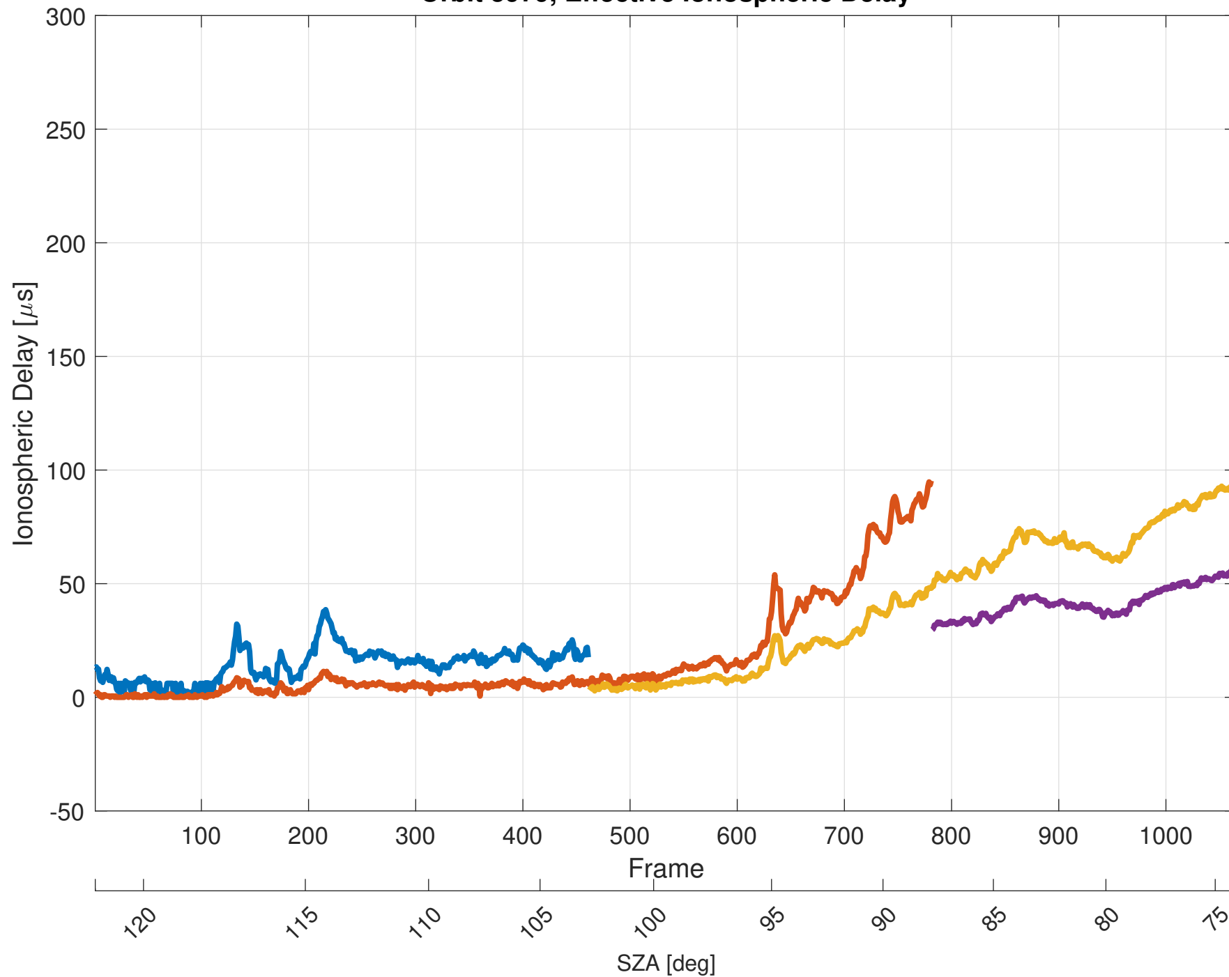
Orbit 5979, Effective Ionospheric Delay
