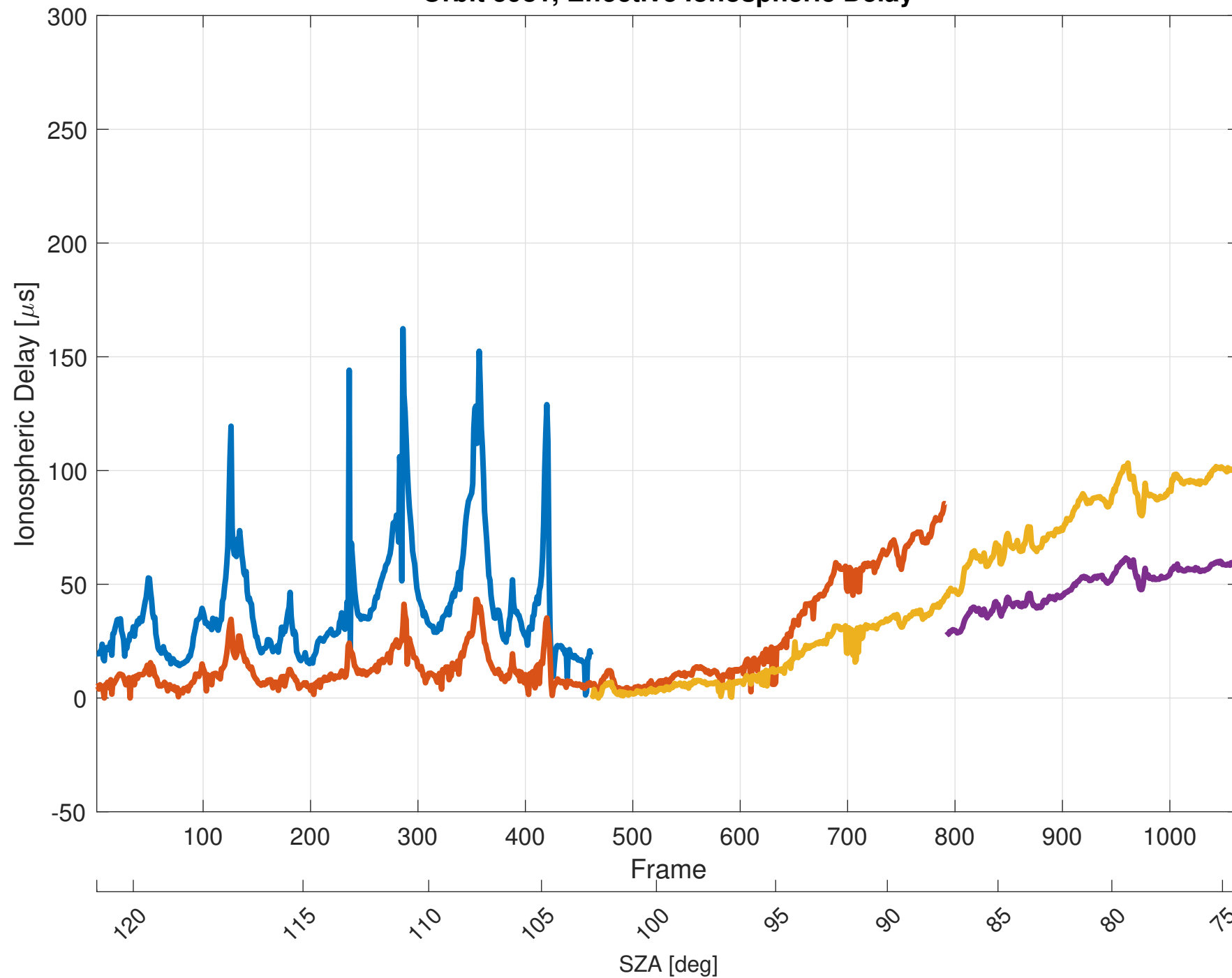
Orbit 5981, Effective Ionospheric Delay
